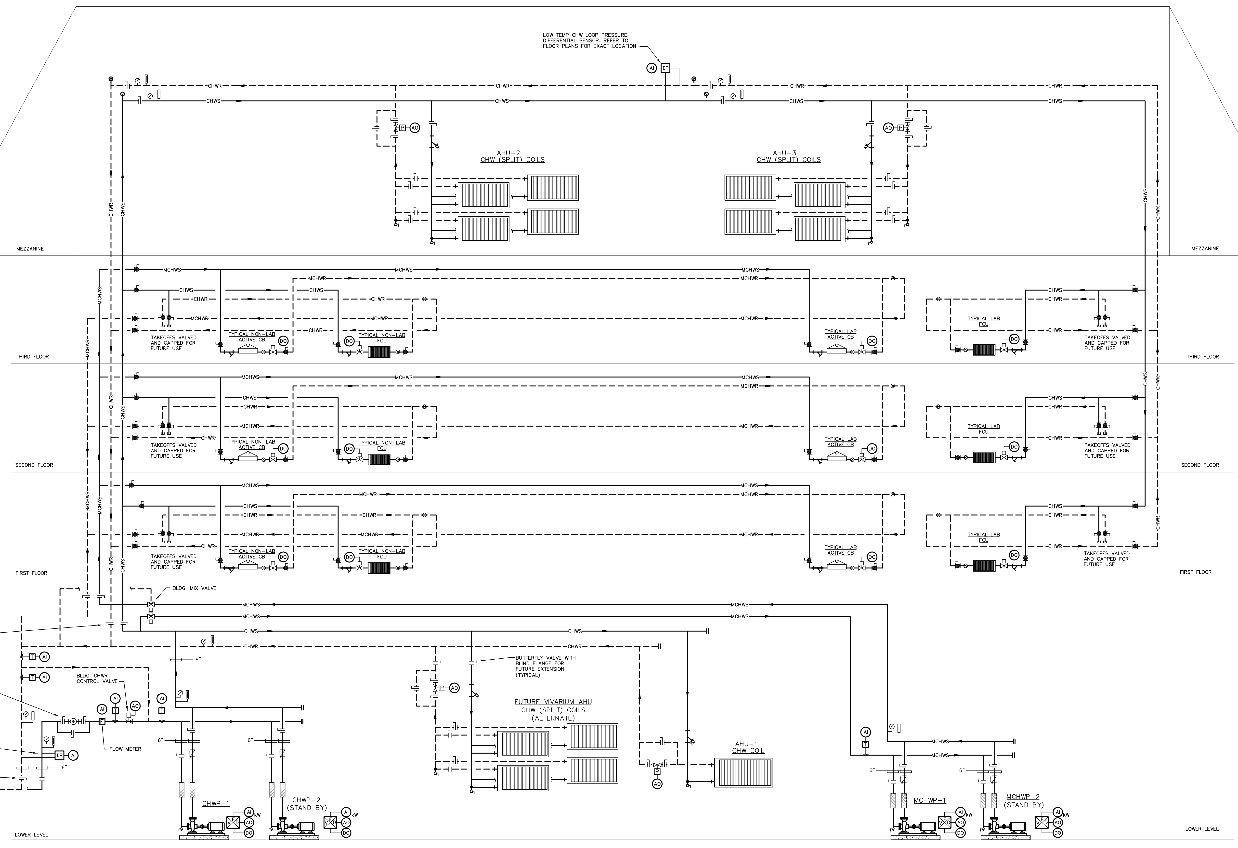
CHILLED WATER RISER DIAGRAM NOT TO SCALE
