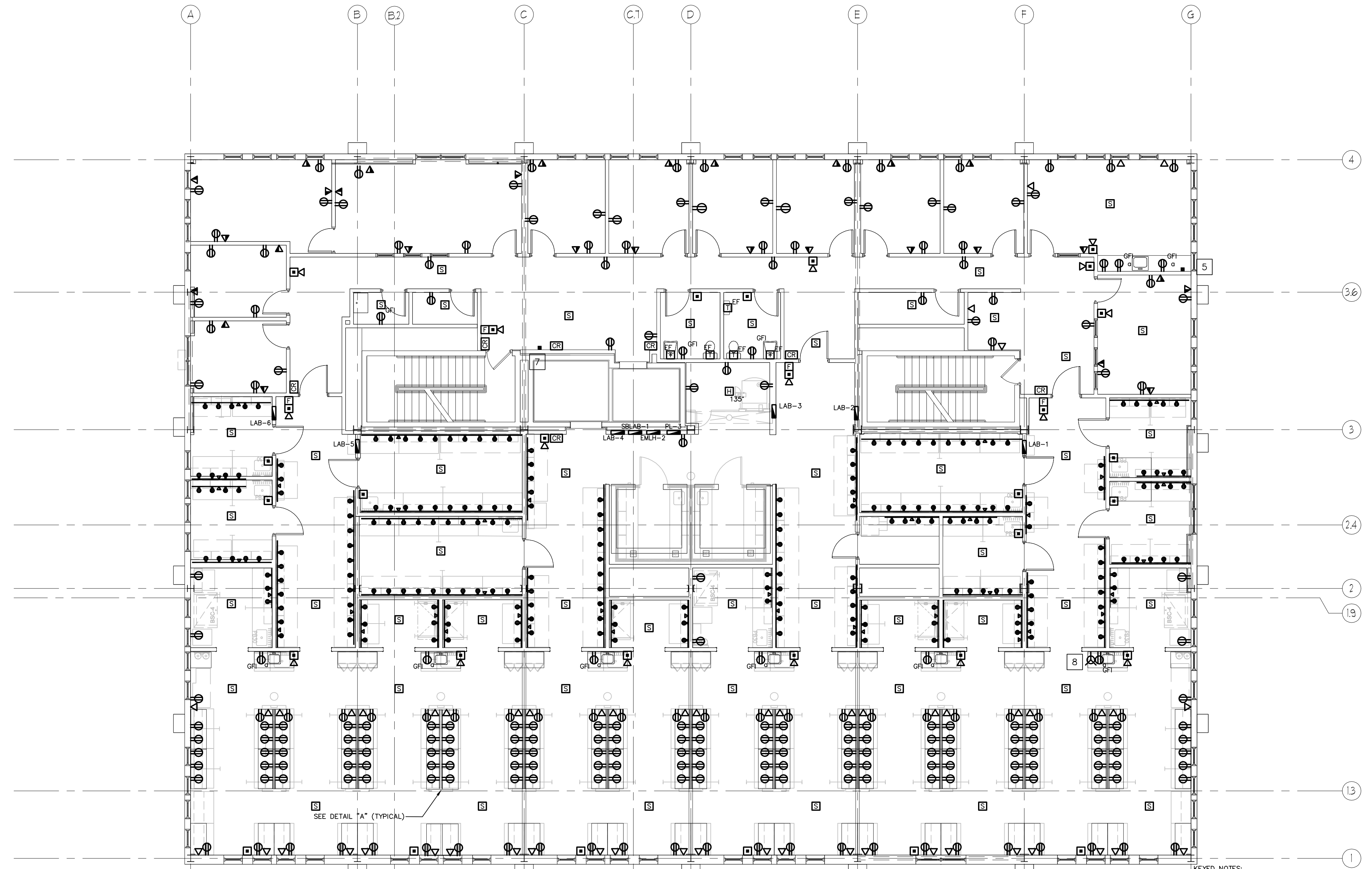
A LAB STATION LAYOUT Scale: 1/4" = 1'
