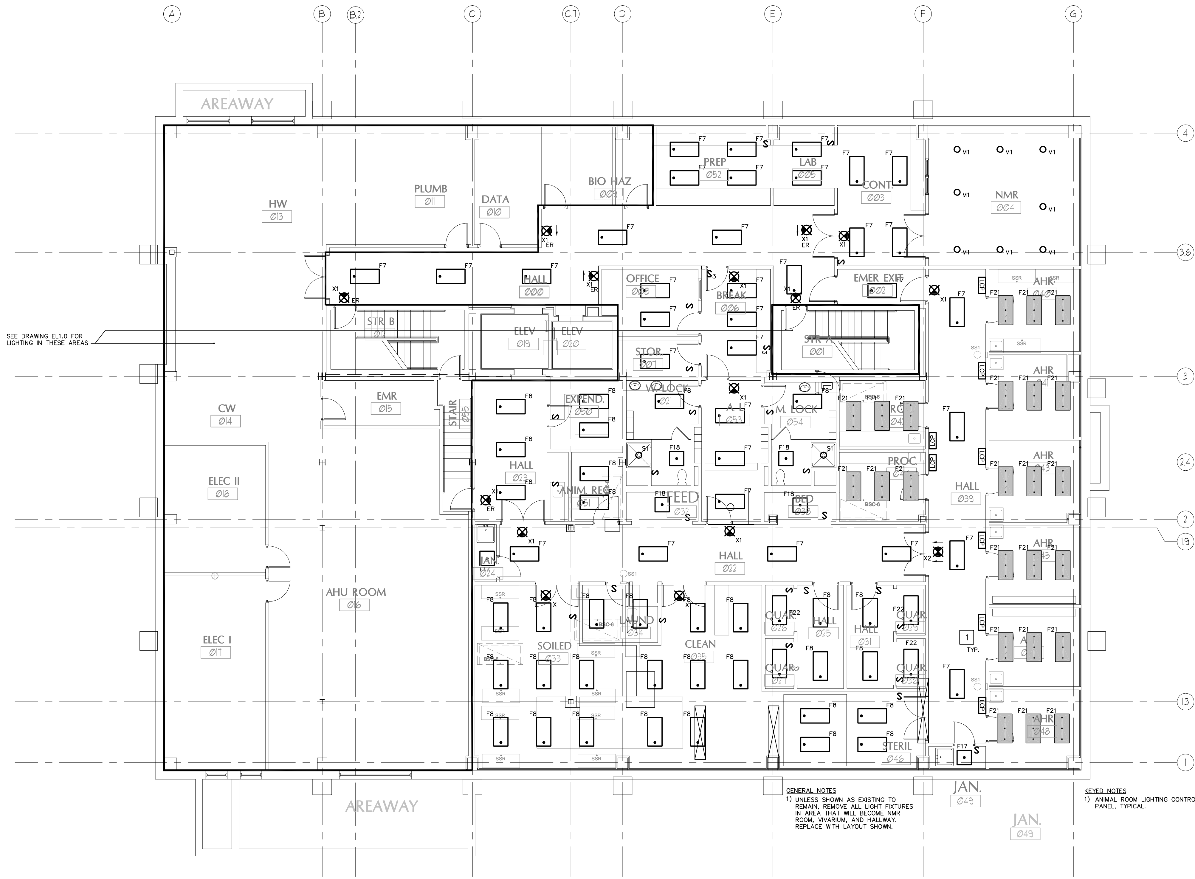
1 LOWER LEVEL LIGHTING PLAN - ALTERNATE Scale: 1/8"=1'-0"
