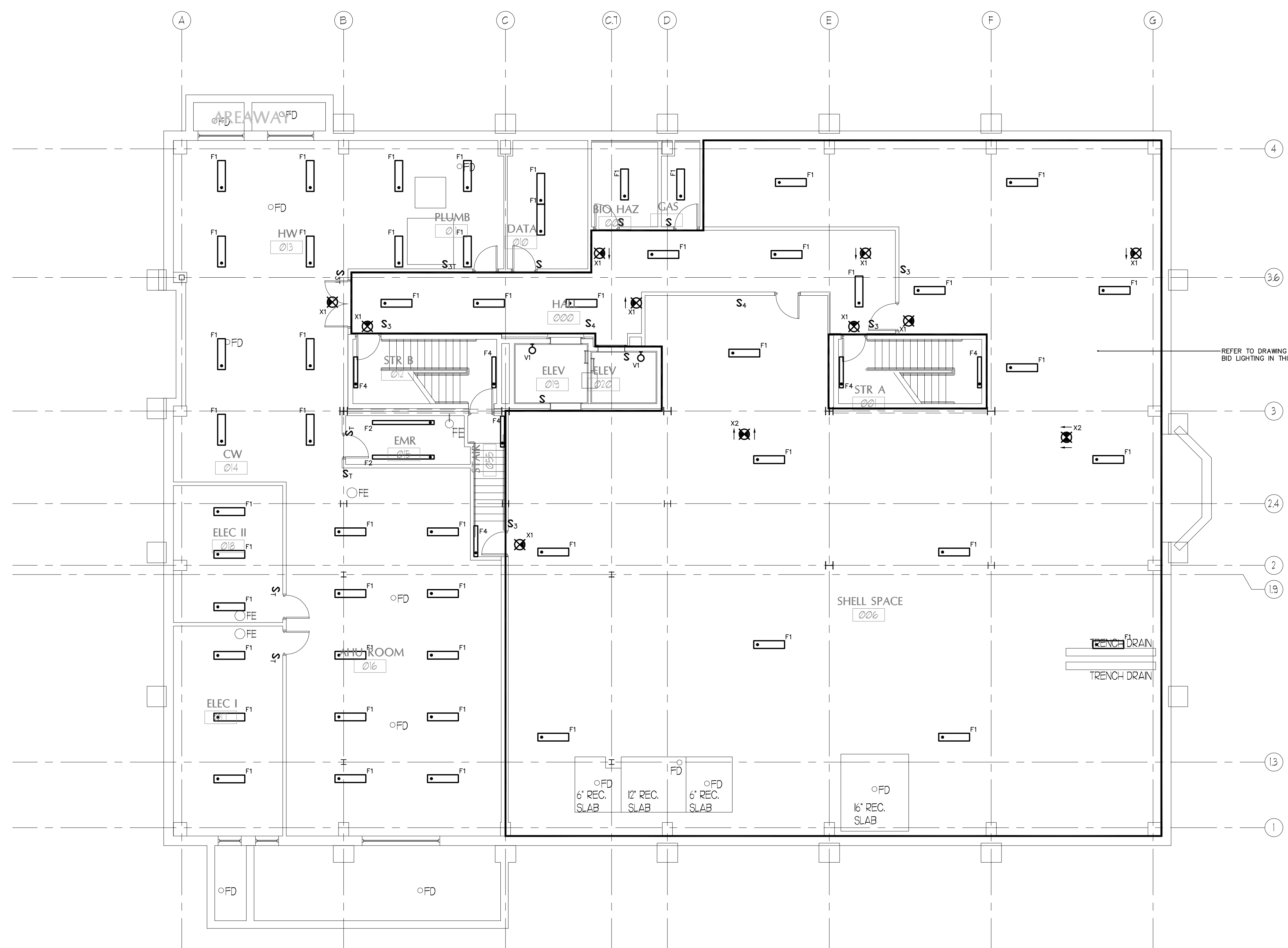
1 LOWER LEVEL LIGHTING PLAN-BASE B ID Scale: 1/8"=1'-0"
