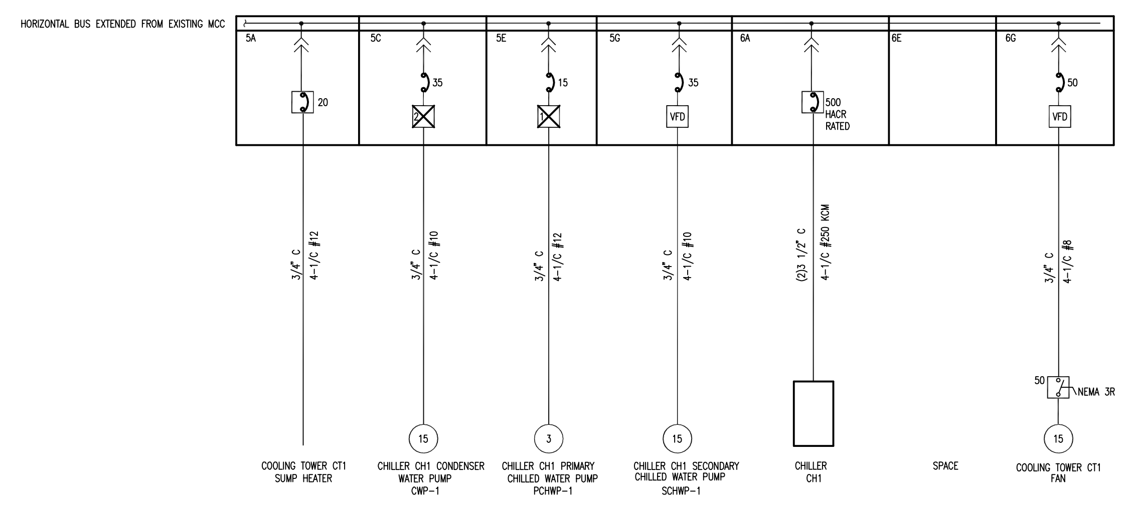
2 NEW MCC SECTIONS RISER DIAGRAM No Scale
