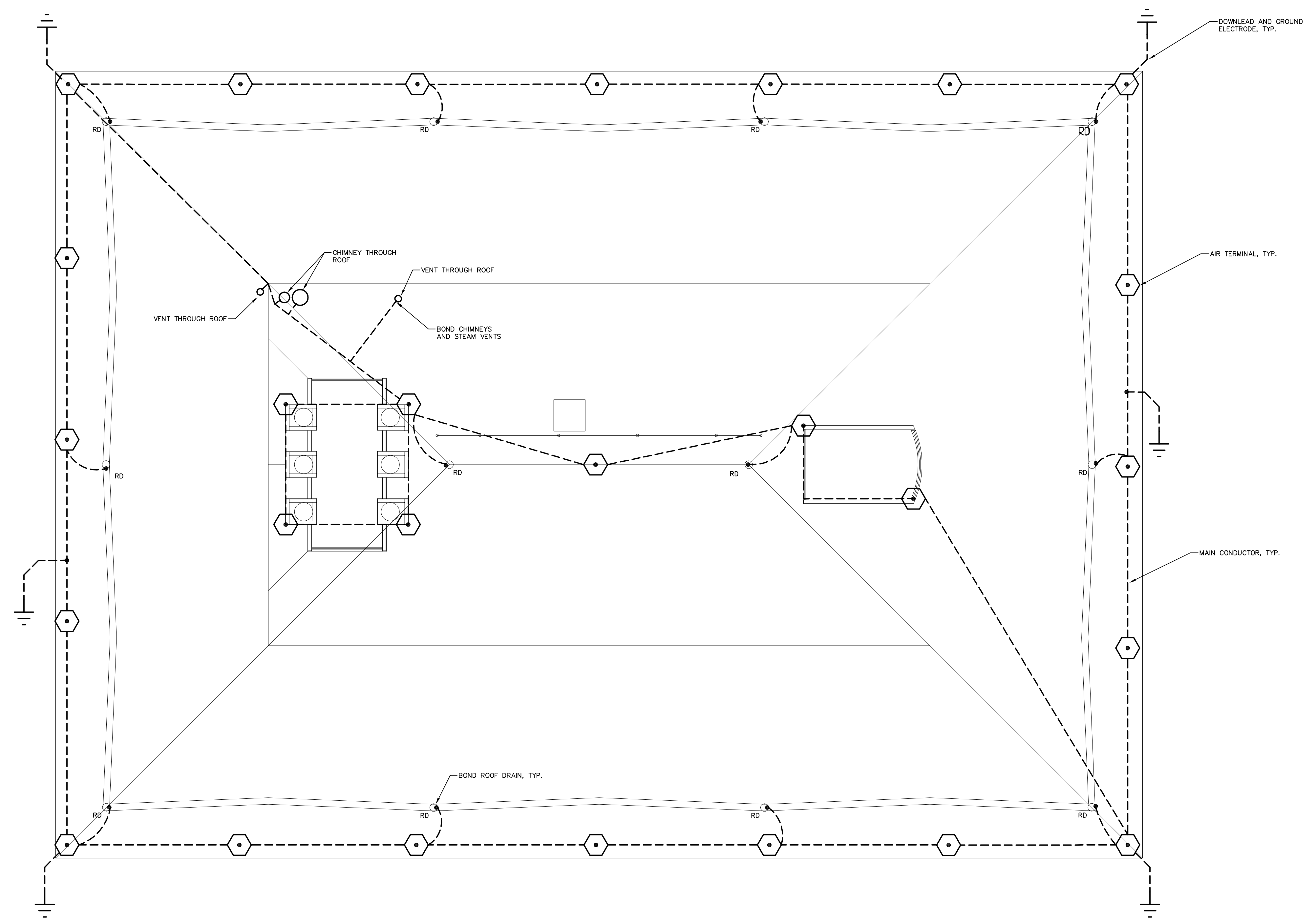
1 LIGHTNING PROTECTION PLAN Scale: 1/8"=1'-0"
