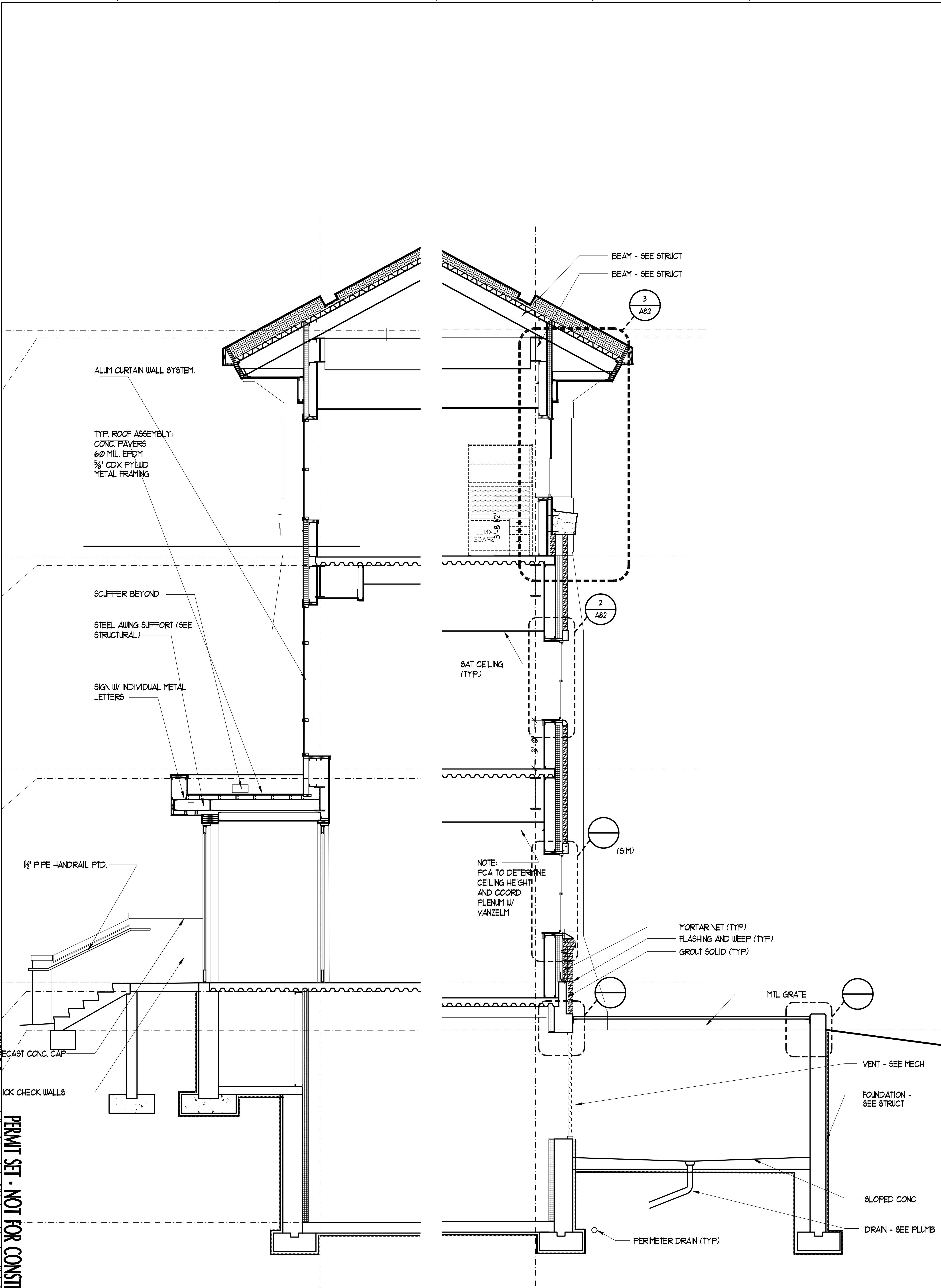
1 WALL SECTION AT FRONT CANOPY SCALE: 3/8" = 1'-0"
