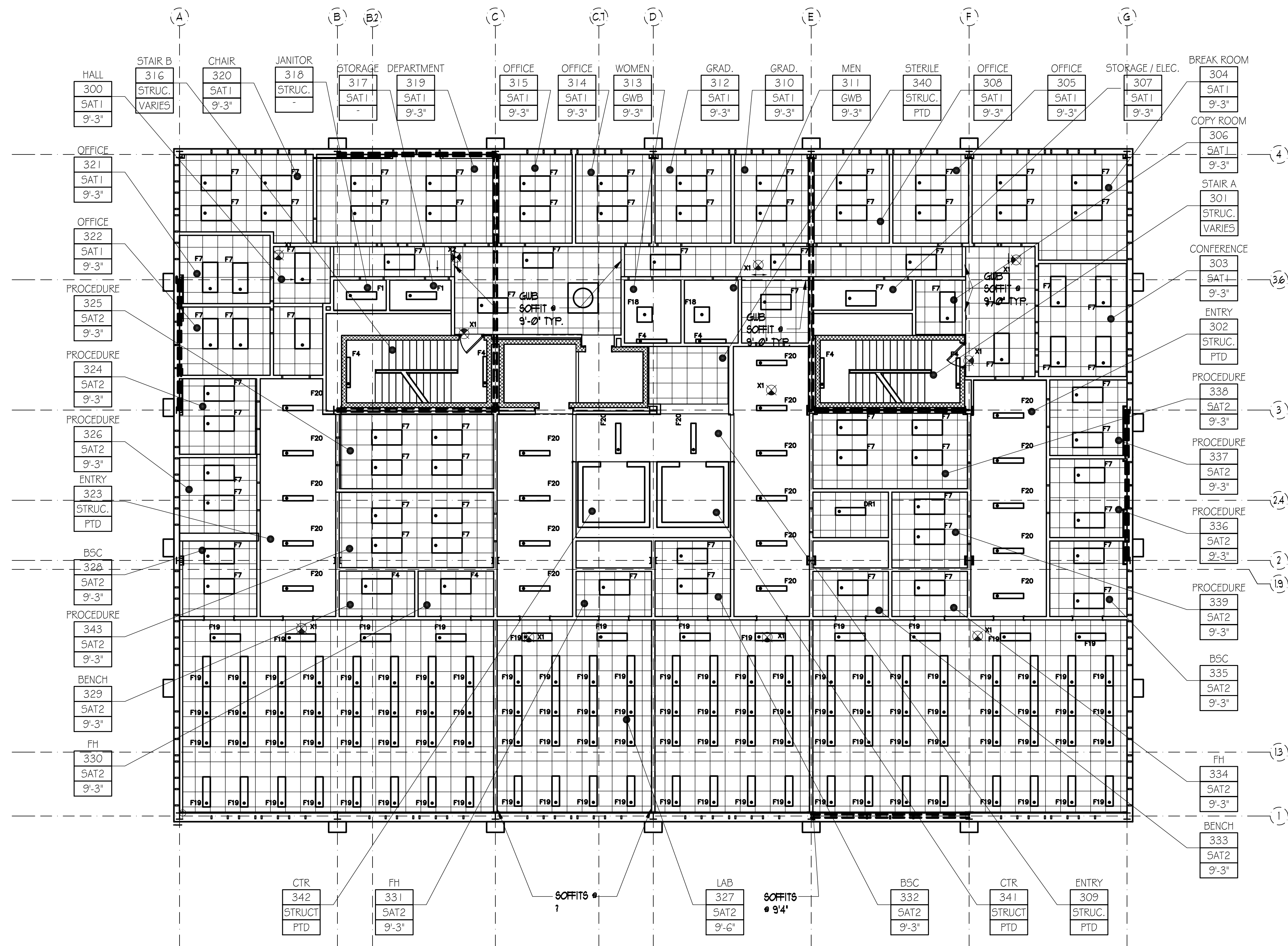
THIRD FLOOR RCP SCALE: 1/8" = 1'-0"
