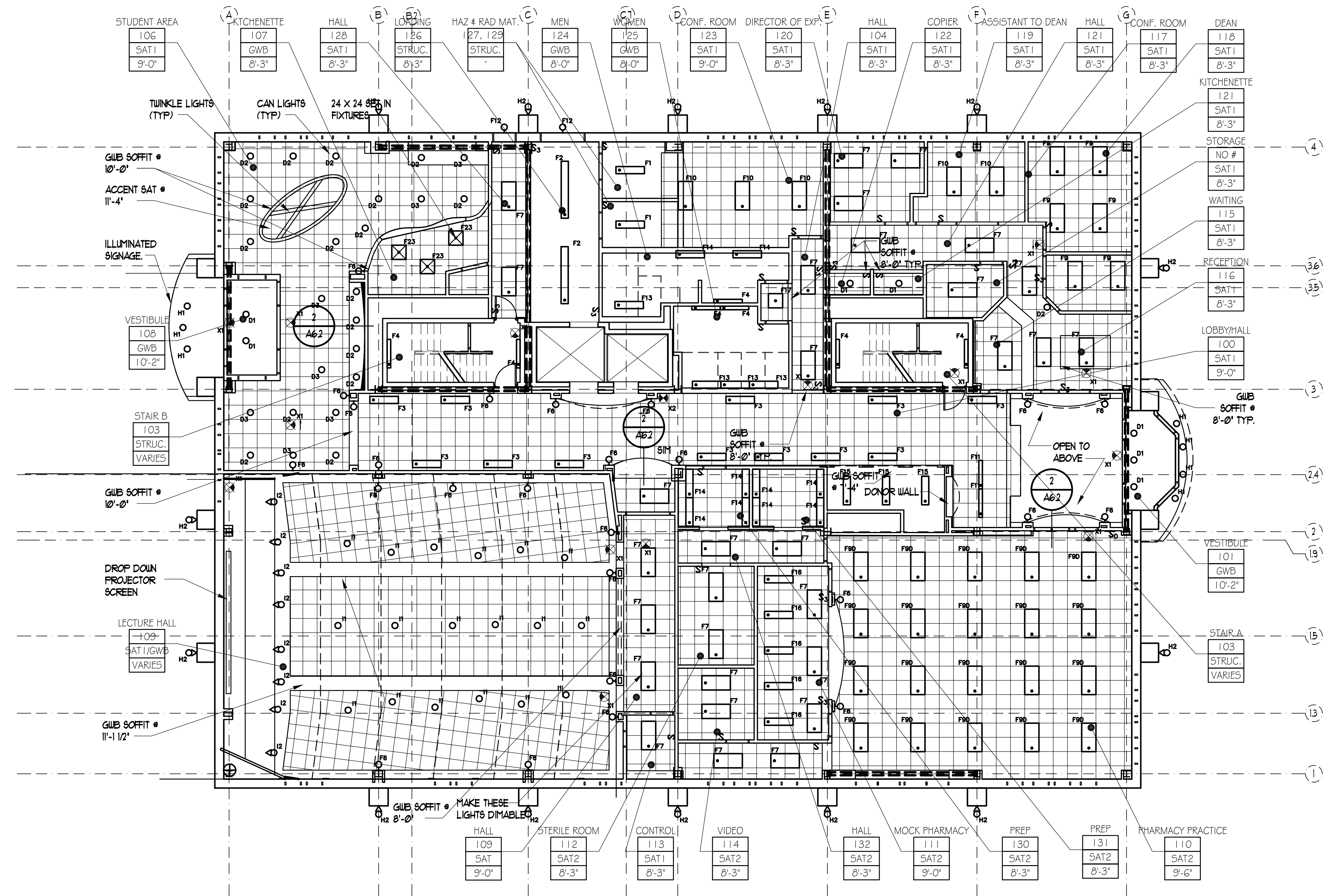
1 FIRST FLOOR RCP A2.2/A2.2 SCALE: 1/8" = 1'-0"
