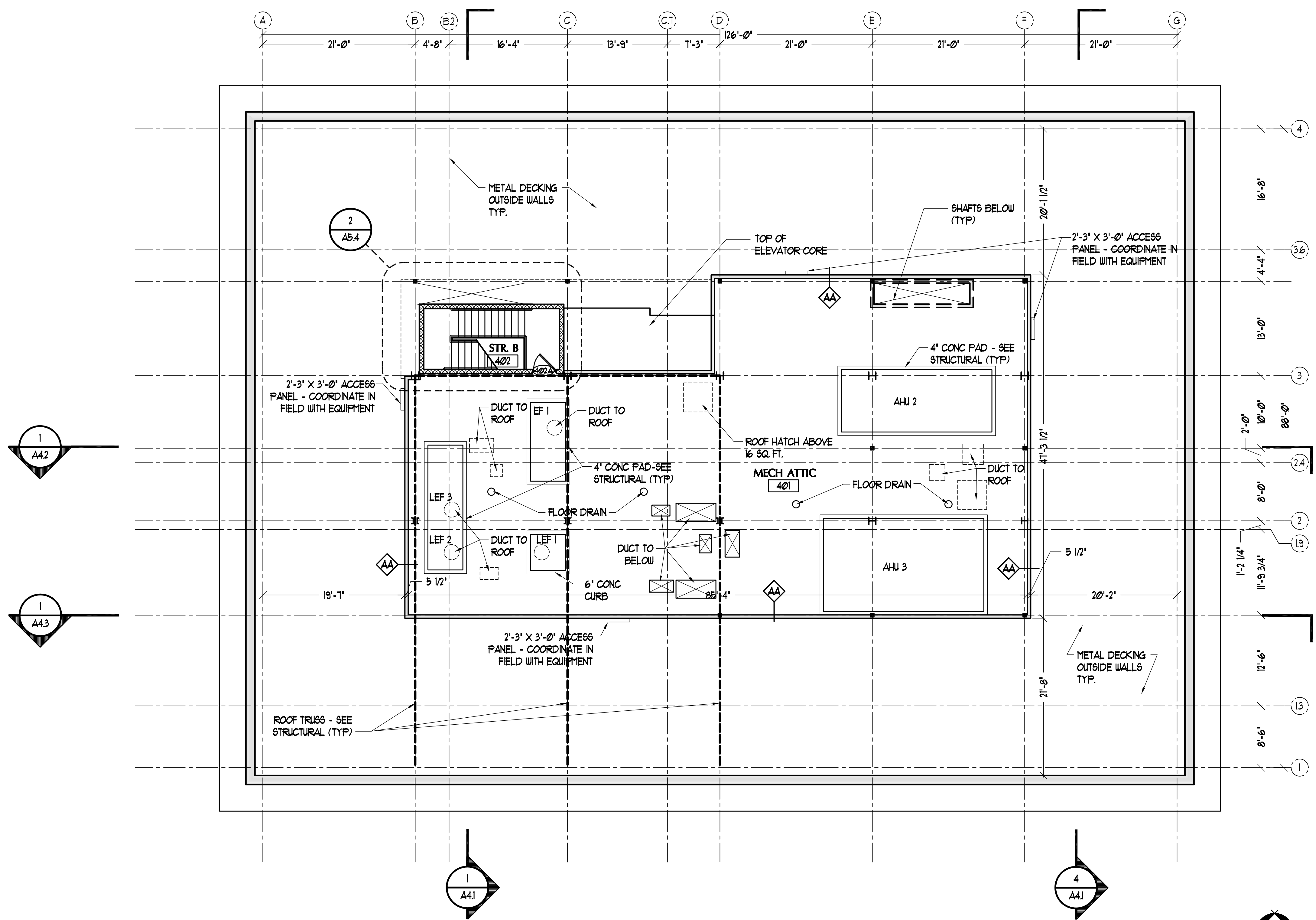
MECHANICAL MEZZANINE SCALE: 1/8" = 1'-0"
