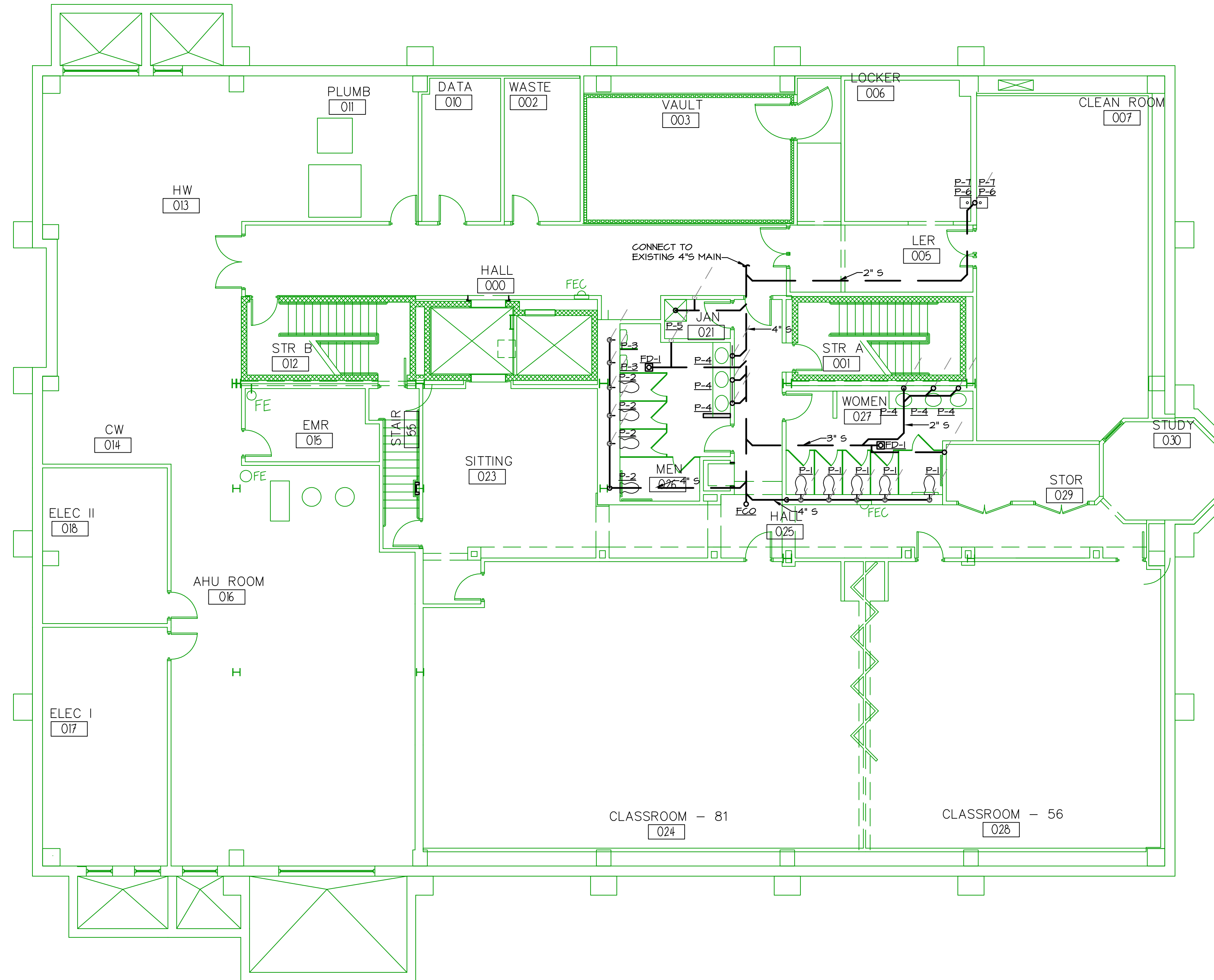
LOWER LEVEL SANITARY PLUMBING PLAN SCALE: 1/8" = 1'-0"
