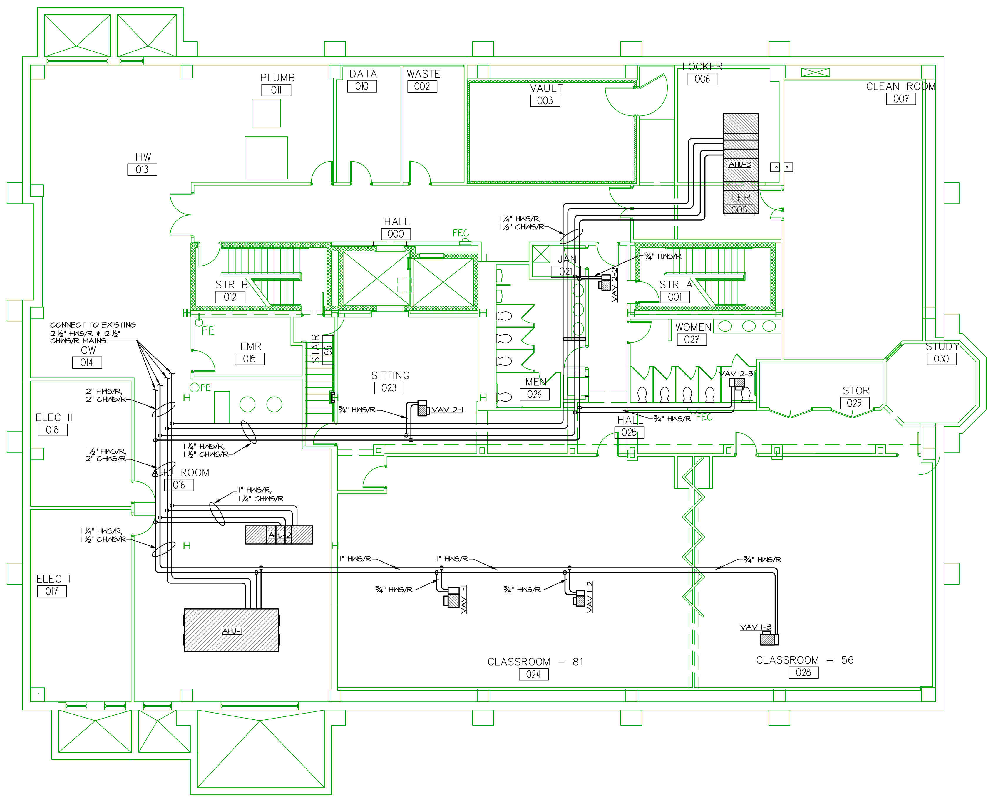
LOWER LEVEL HVAC PIPING PLAN SCALE: 1/8" = 1'-0"
