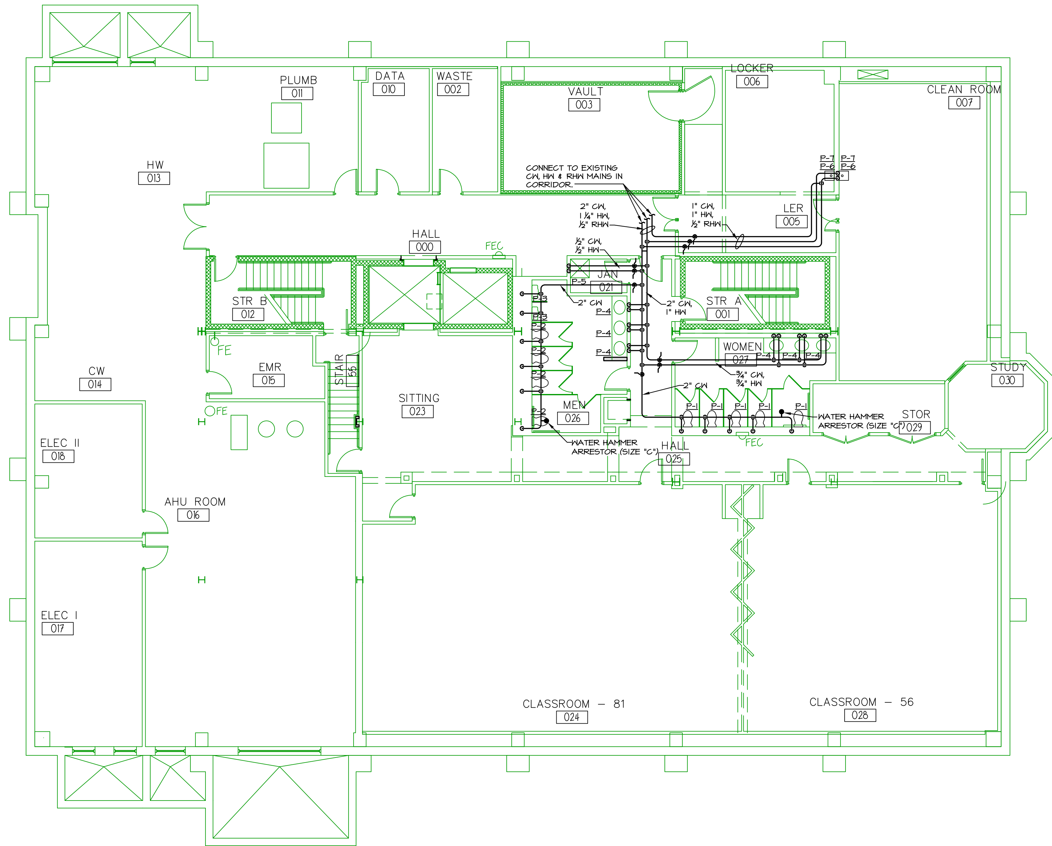
LOWER LEVEL DOMESTIC PLUMBING PLAN SCALE: 1/8" = 1'-0"
