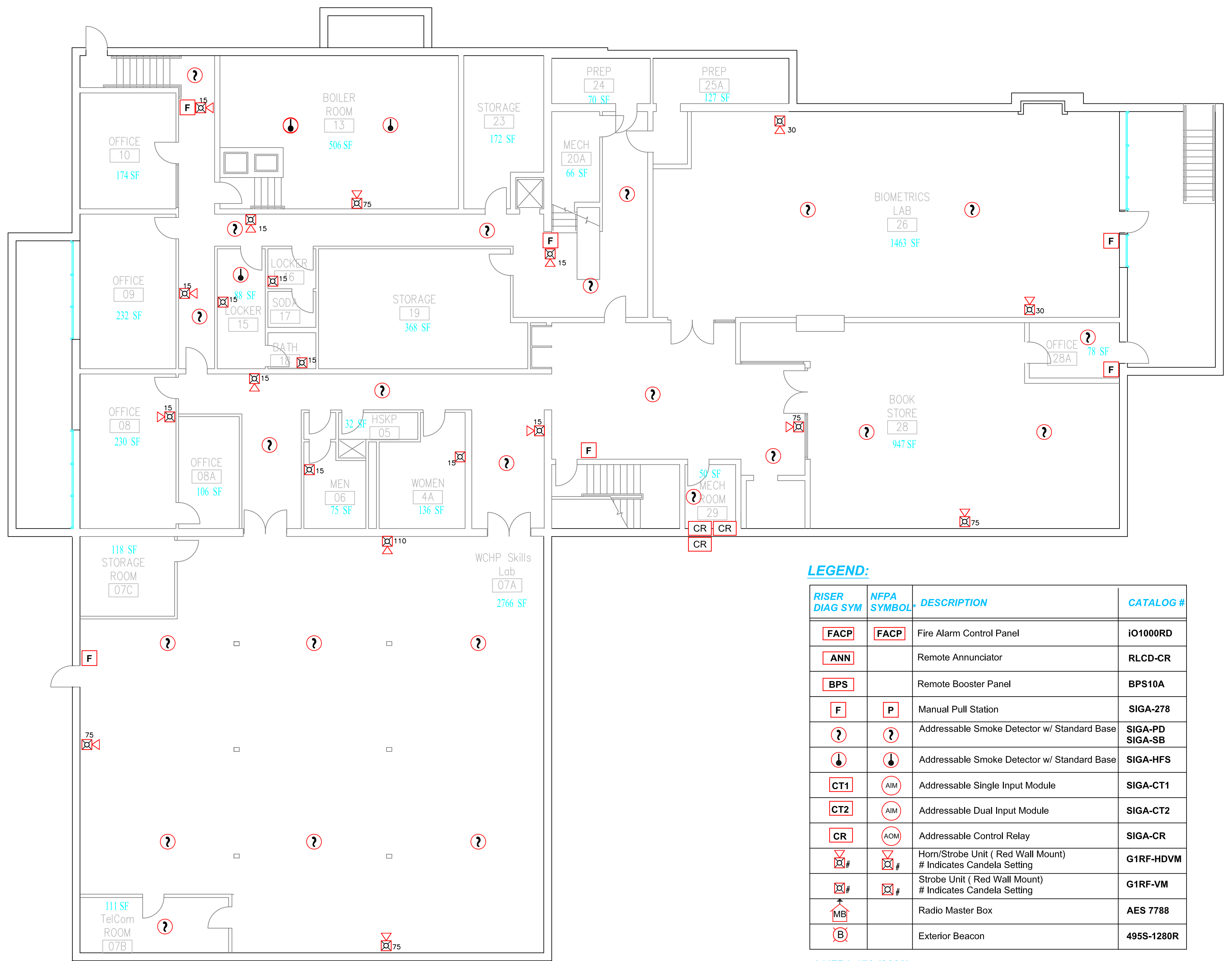
1 LOWER LEVEL PLAN SCALE: 1/8" = 1'-0"
