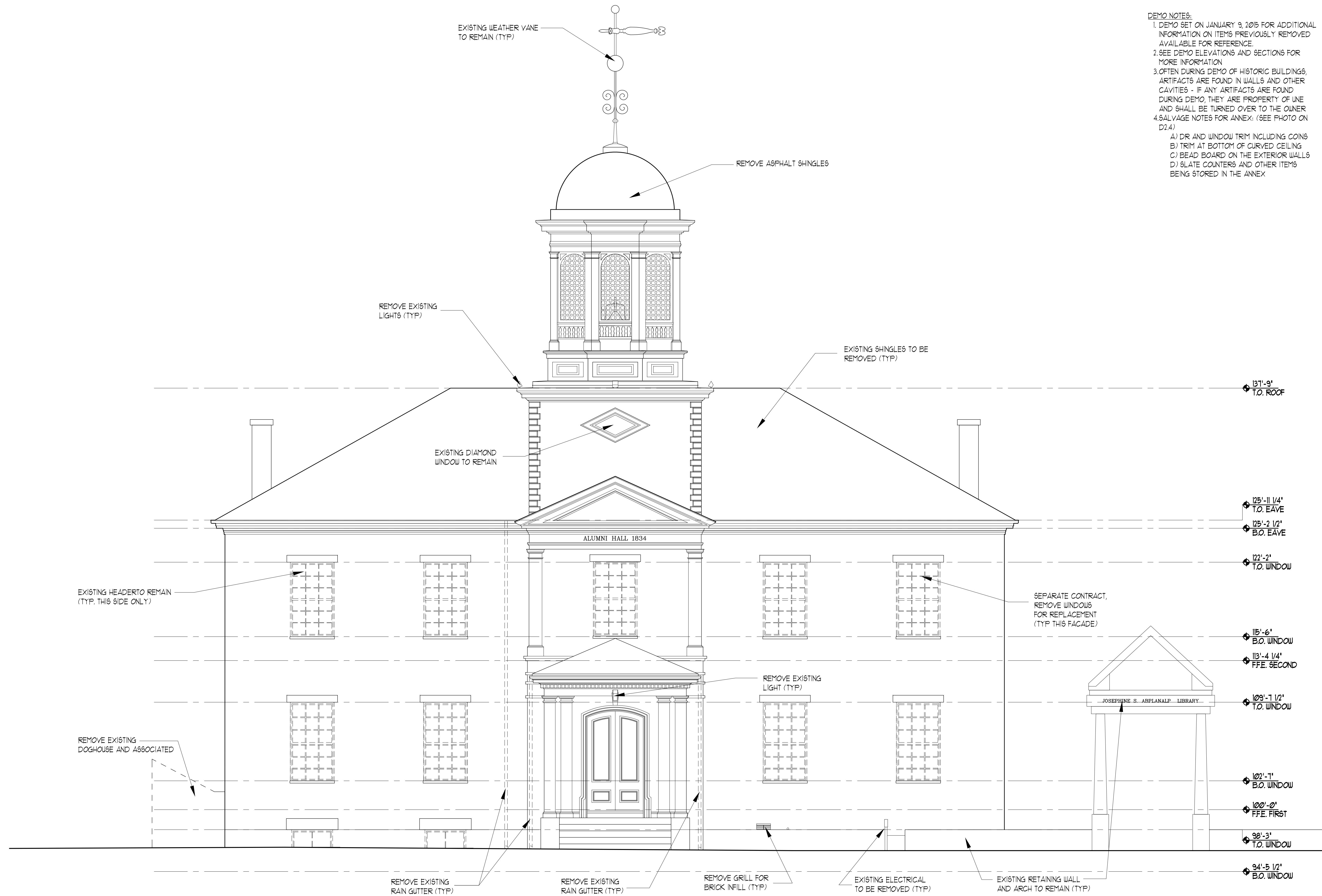
1 EXISTING EAST ELEVATION SCALE: 1/4" = 1'-0"
