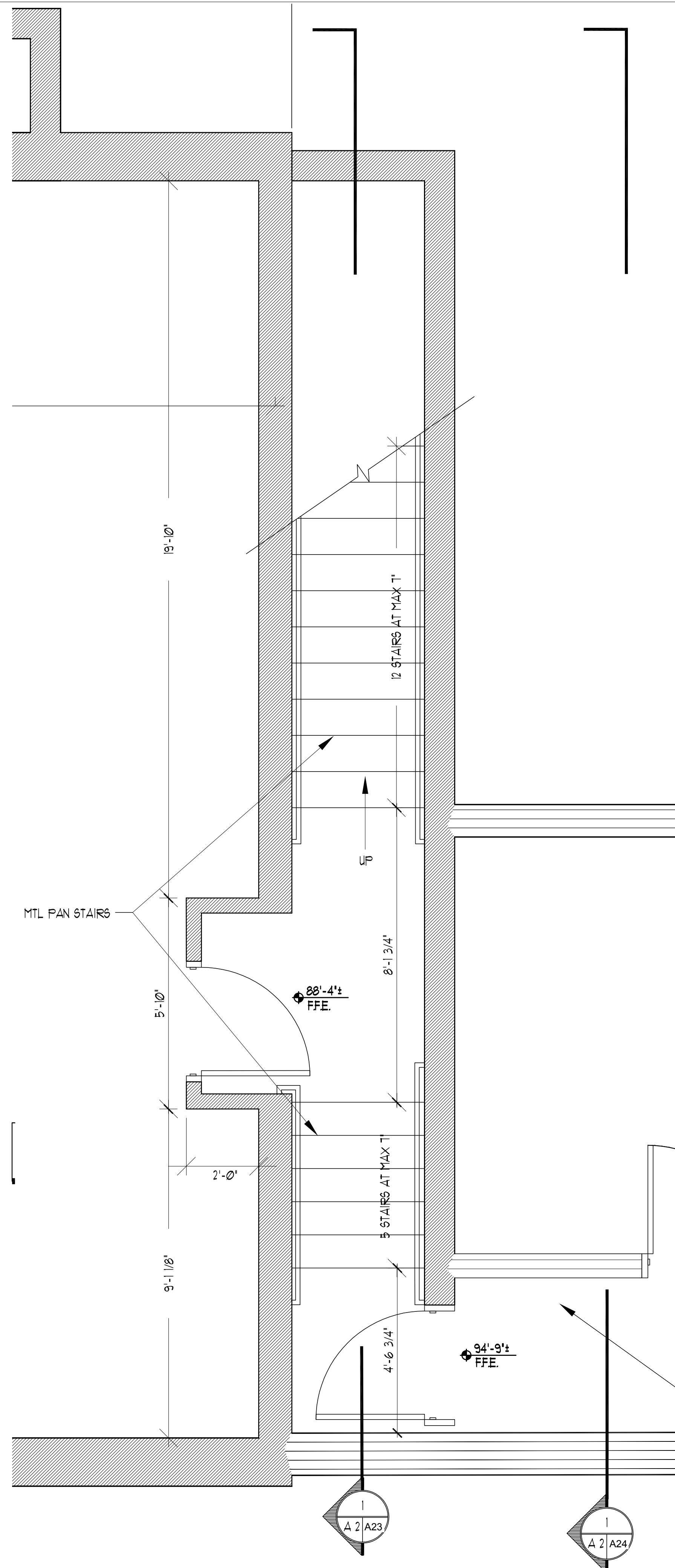
2 LOWER LEVEL STAIR PLAN SCALE: 1/2" = 1'-0"
