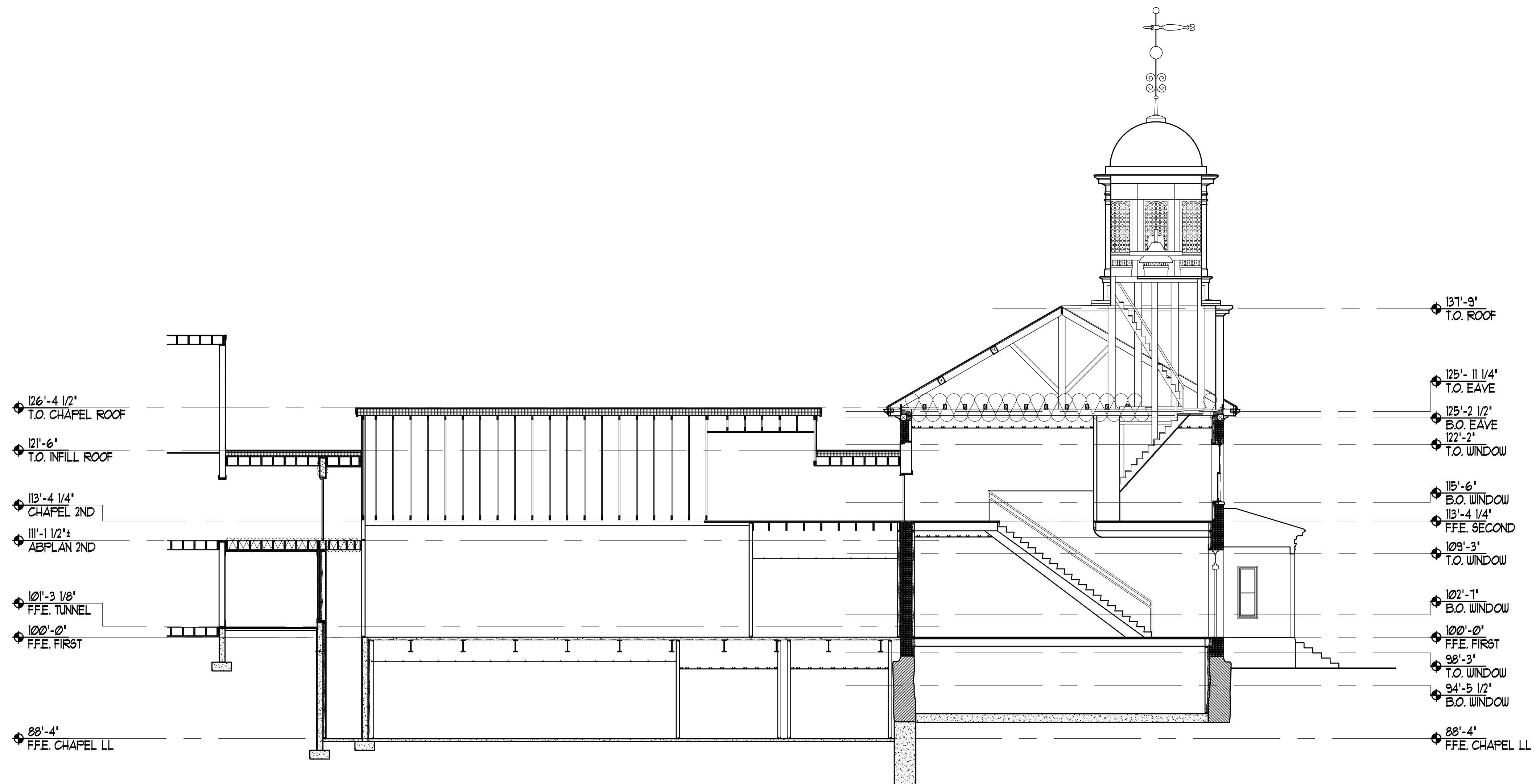
1 ALUMNI/ CHAPEL SECTION SCALE: 1/8" = 1'-0"
