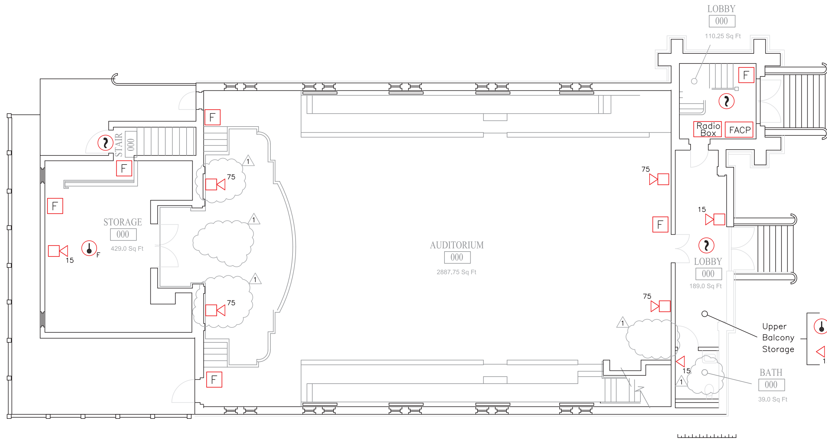
Upper Level Plan
