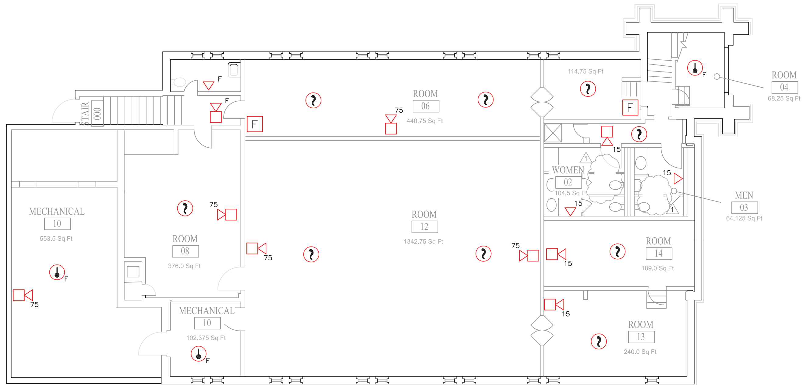
Lower Level Plan
