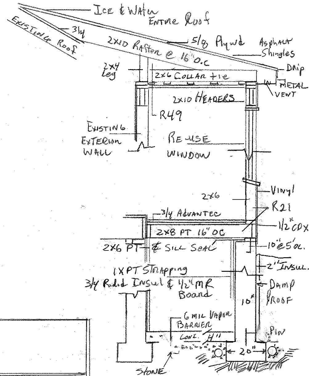
① CELLAR ENTRY DETAIL SCALE 3/8" = 1'-0"
