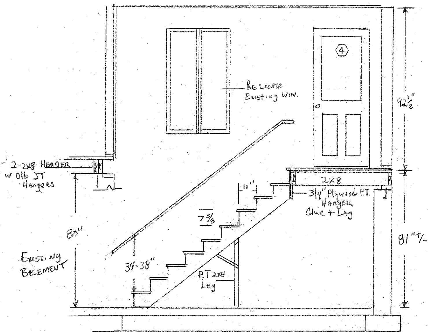
NEW CELLAR ENTRY DETAIL SCALE 3/8" = 1'-0"
