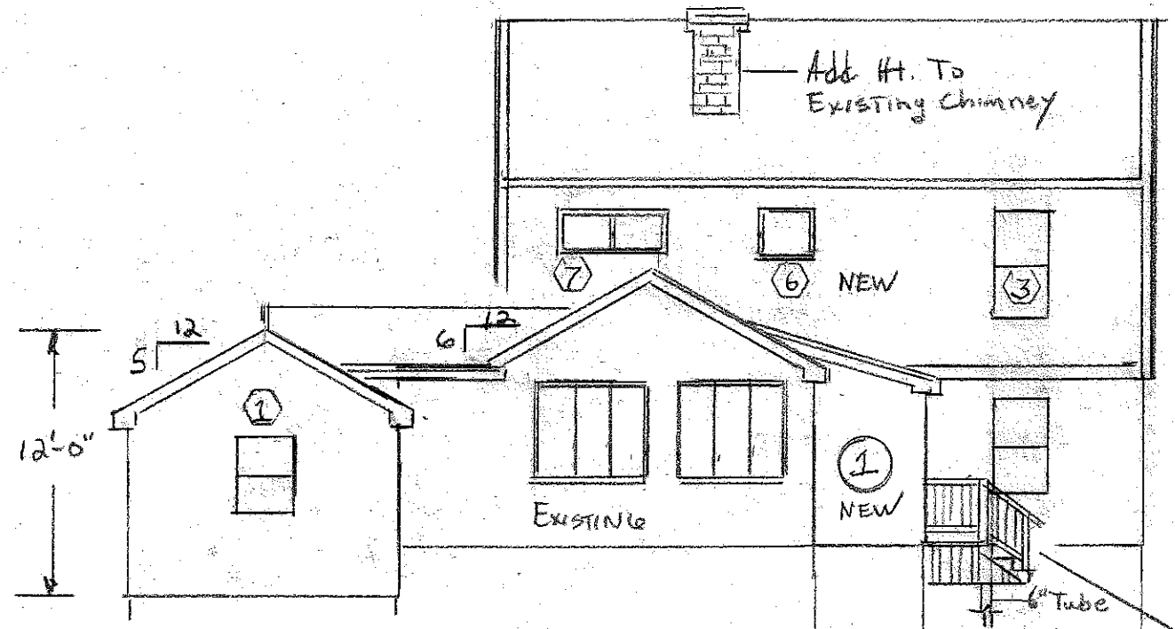
NEW REAR ELEVATION SCALE 1/8" = 1'-0"
