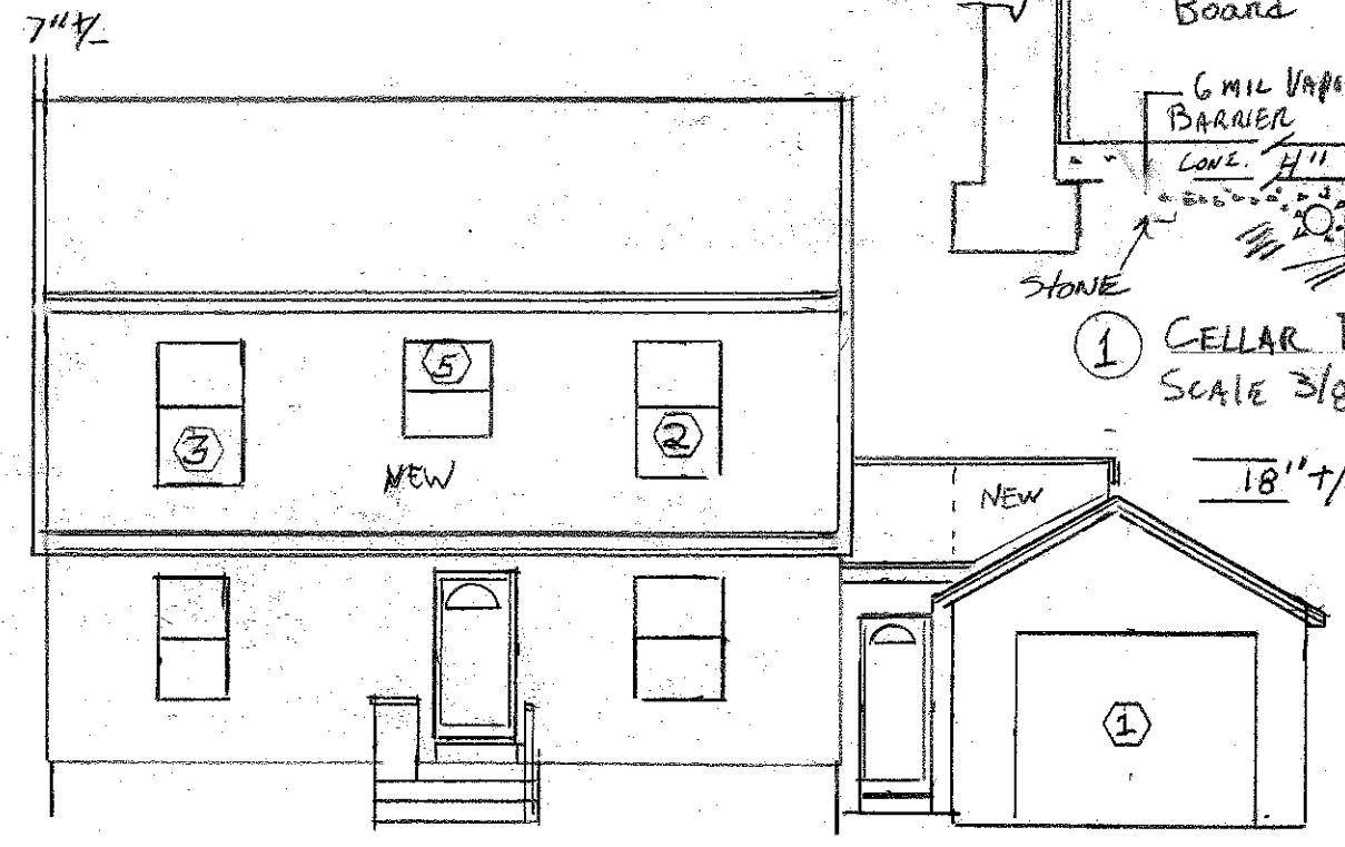
NEW FRONT ELEVATION SCALE 1/8" = 1'-0"
