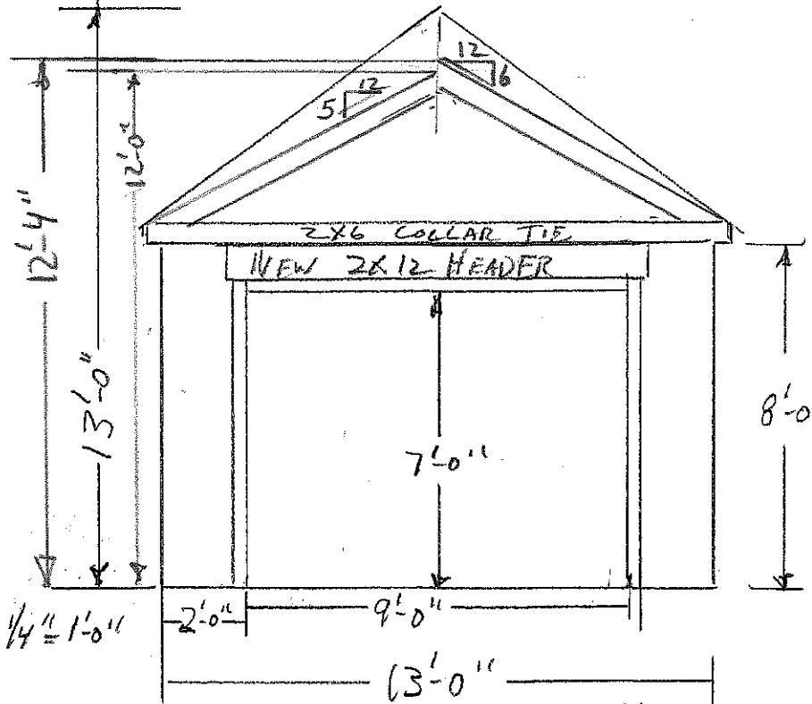
NEW GARAGE PLAN
