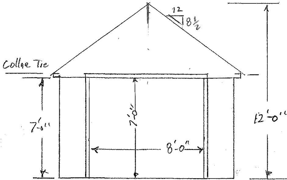
EXISTING GARAGE
