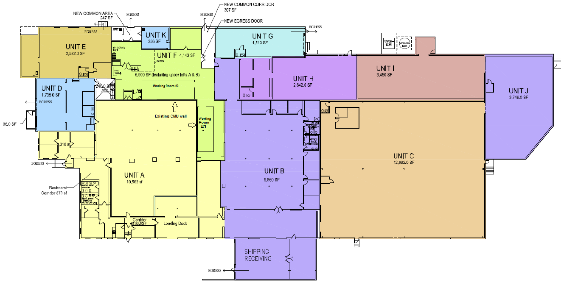
135 Walton Street Portland, Maine Ground Level Plan
