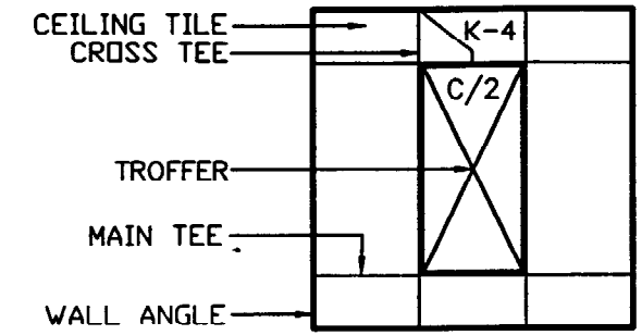
CEILING PLAN
