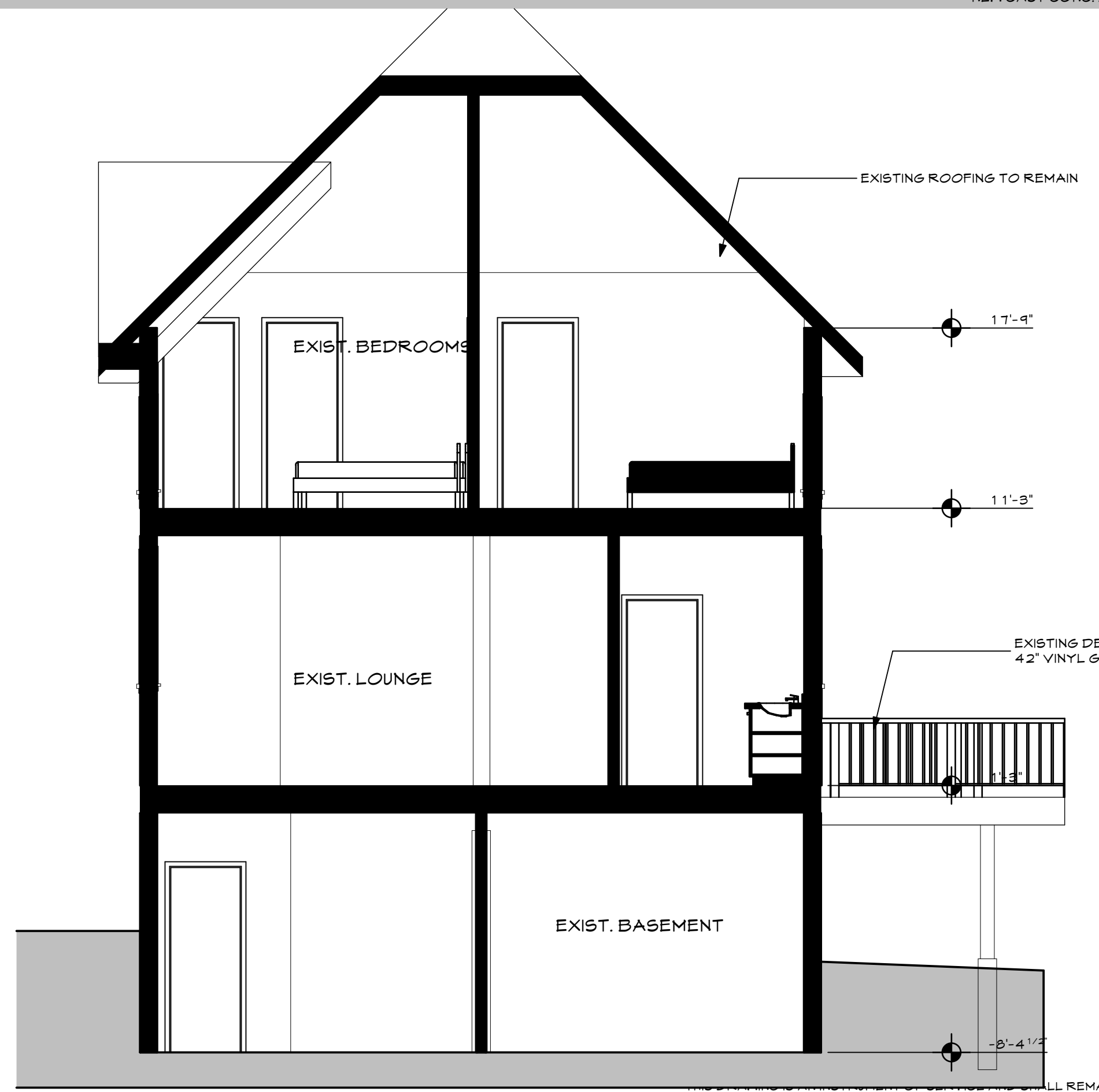
1 Building Section A A3.1 SCALE: 1/4" = 1'-0"
