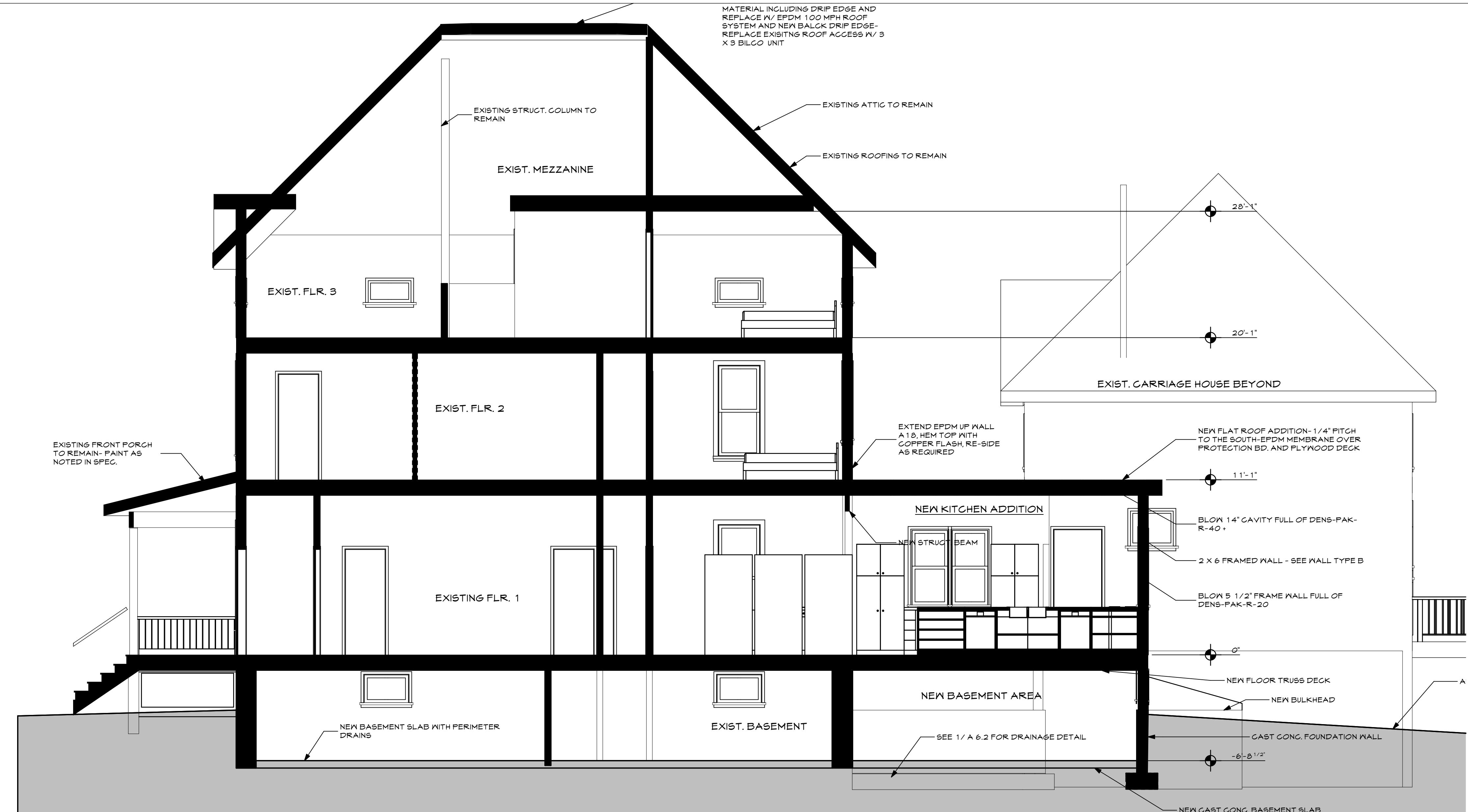
1 Building Section A A3.1 SCALE: 1/4" = 1'-0"
