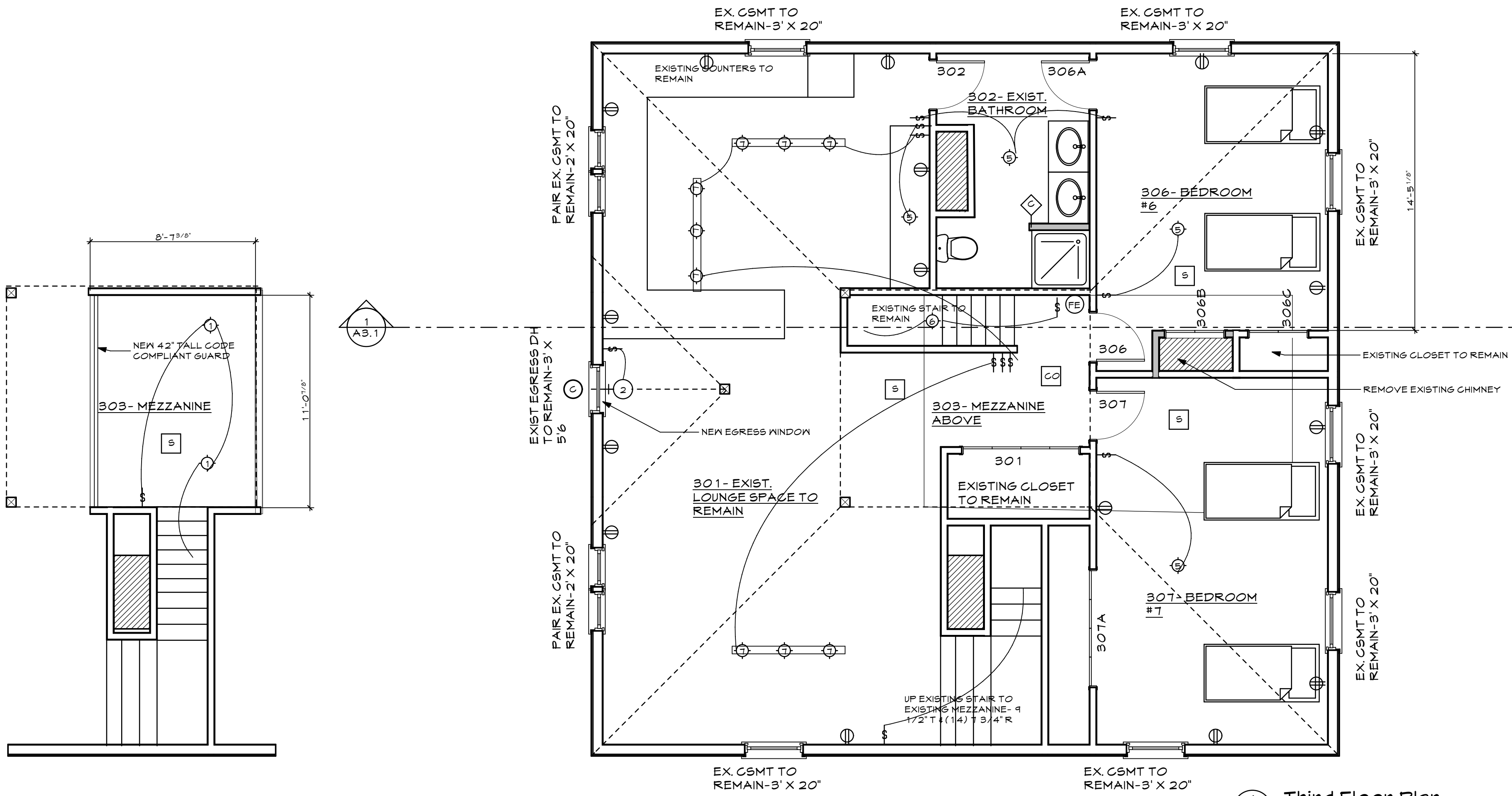
1 Third Floor Plan A1.4 SCALE: 1/4" = 1'-0"
