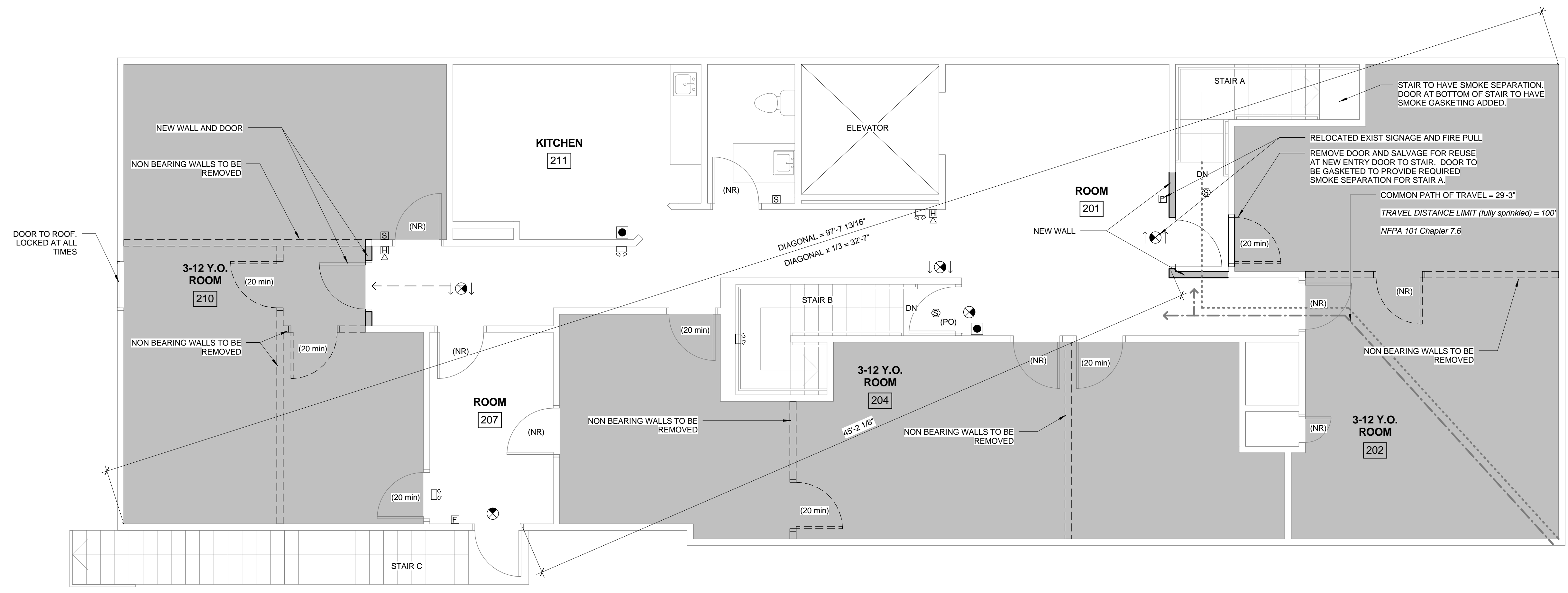
1 | 2ND FLOOR - LIFESAFETY 1/4" = 1'-0"
