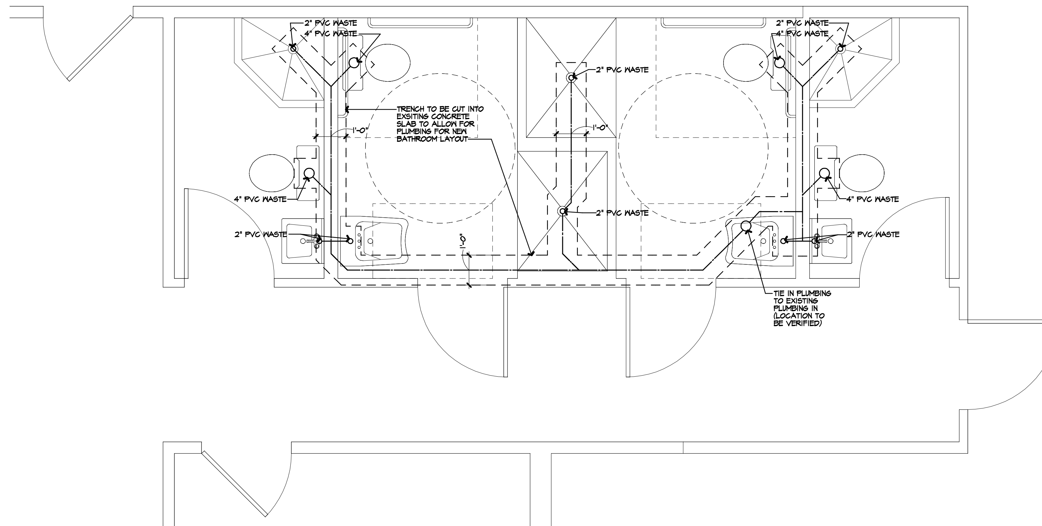
1 BATHROOM PLUMBING PLAN P-1 1/2" = 1'-0" 1 2 4 8
