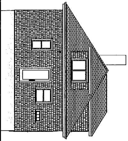
Rear Elevation : 1/8 in = 1 ft
