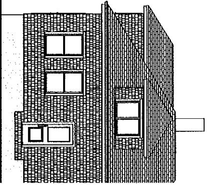
Side Elevation : 1/8 in = 1 ft
