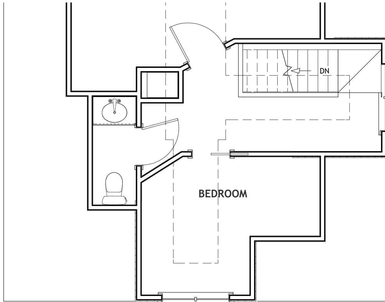
2nd Floor : 1/4 in = 1 ft
