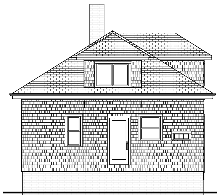
Rear Elevation : 1/8 in = 1 ft
