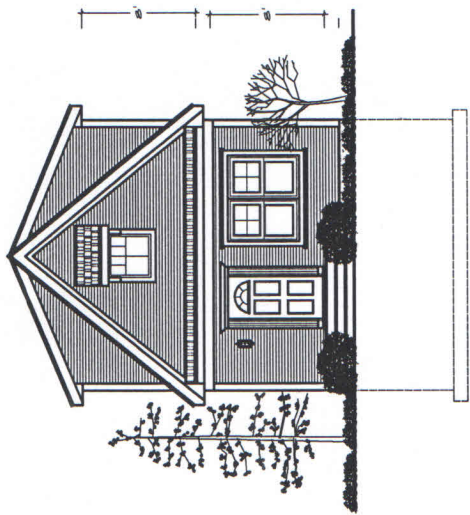
FRONT ELEVATION 1/4"=1'-0"
