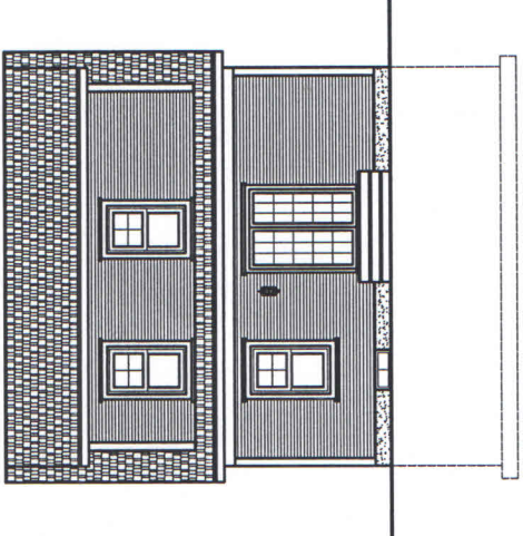
RIGHT ELEVATION 1/4"=1'-0"
