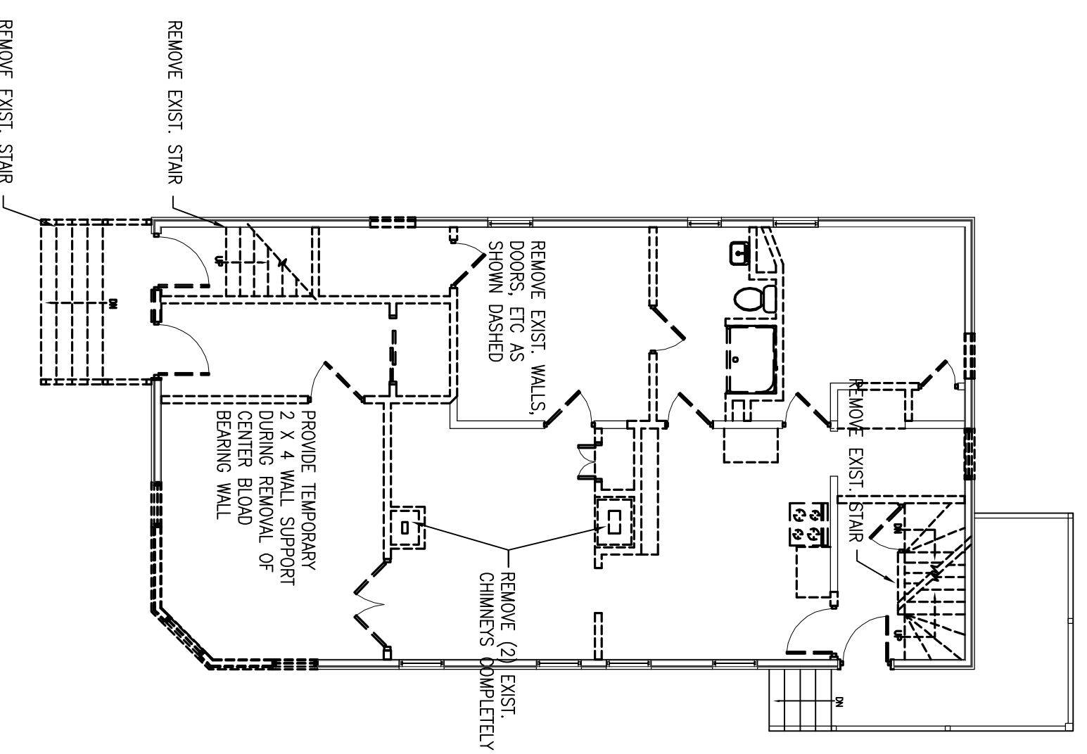
FIRST FLOOR DEMO PLAN SCALE: 1/8" = 1'-0"
