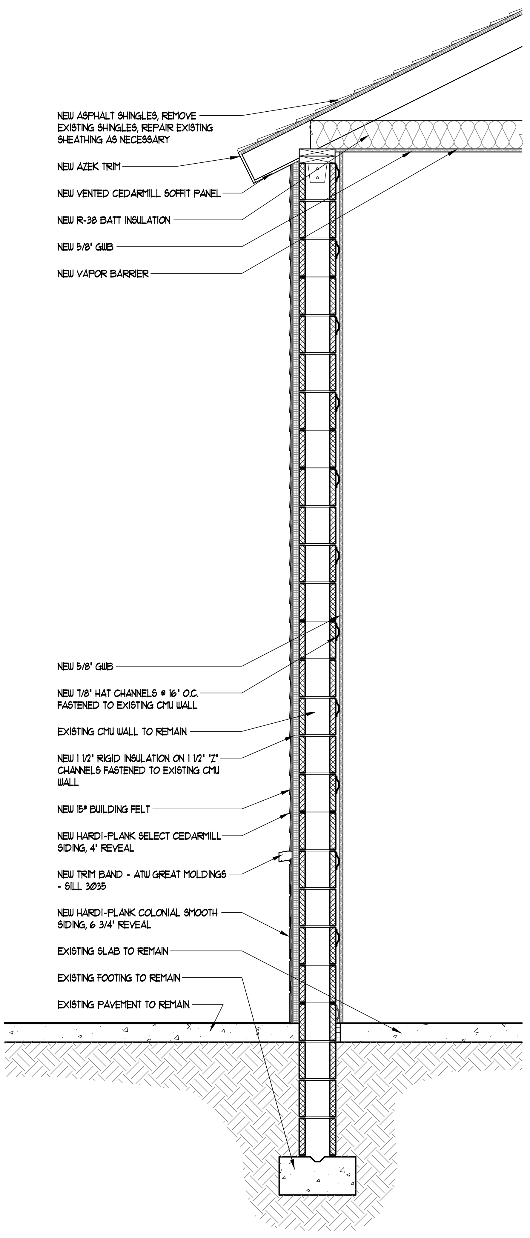
TYPICAL WALL SECTION SCALE: 1" = 1'-0"
