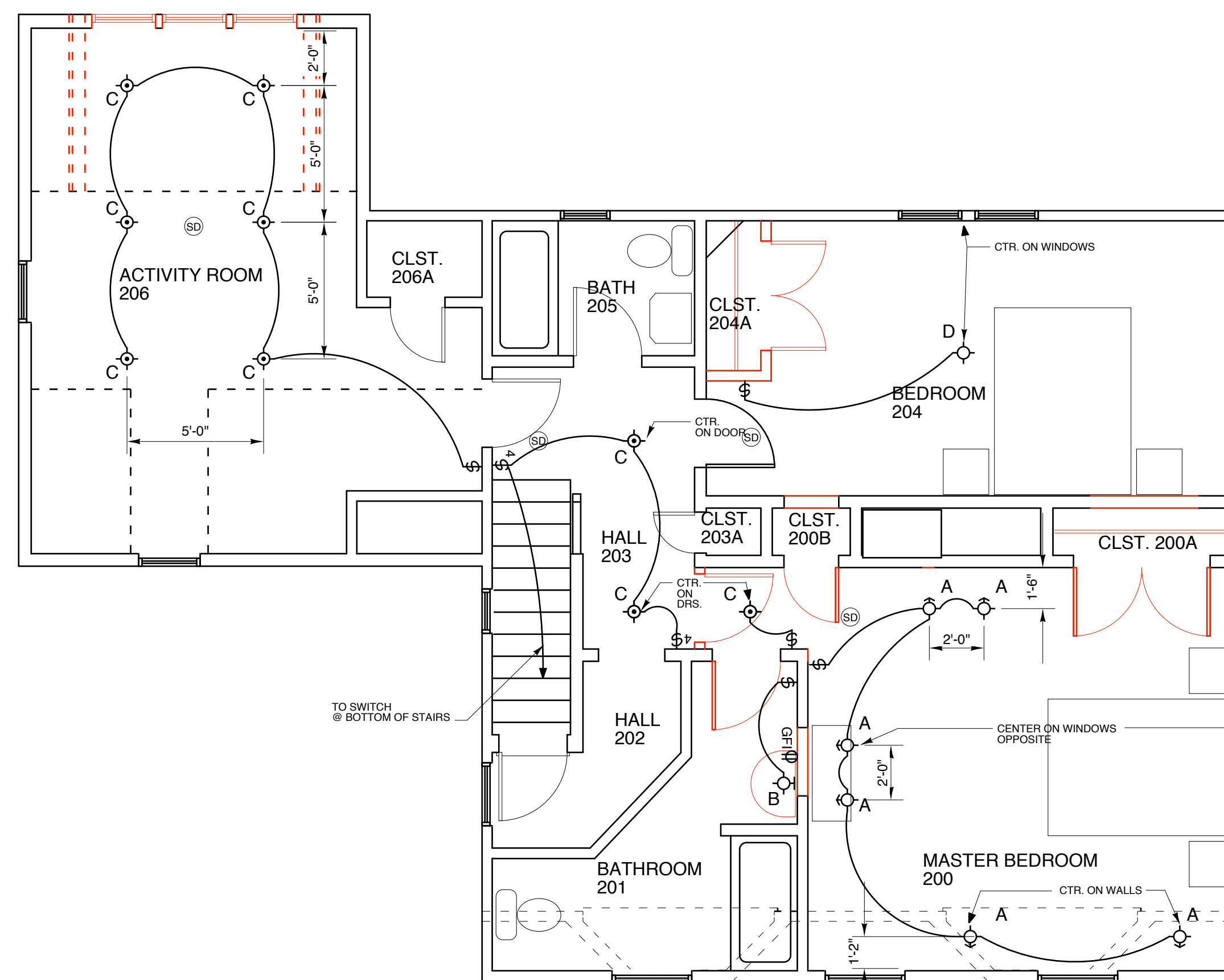
SECOND FLOOR
