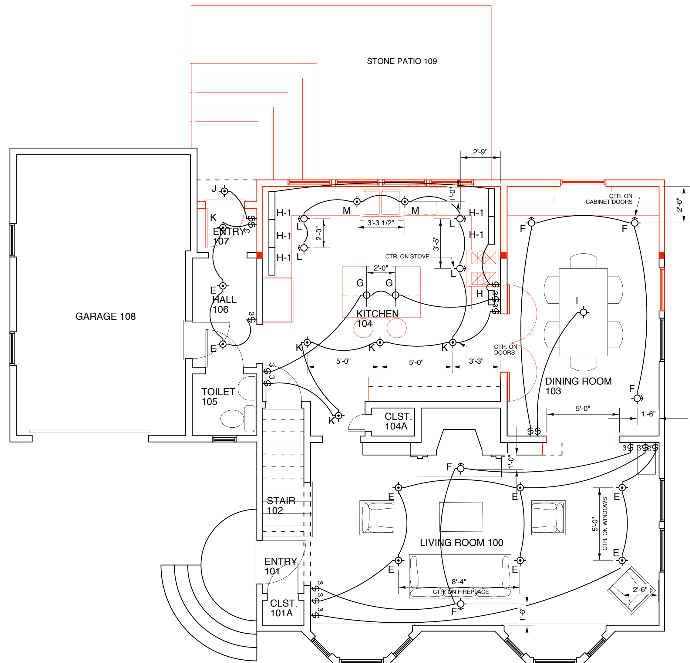
FIRST FLOOR
