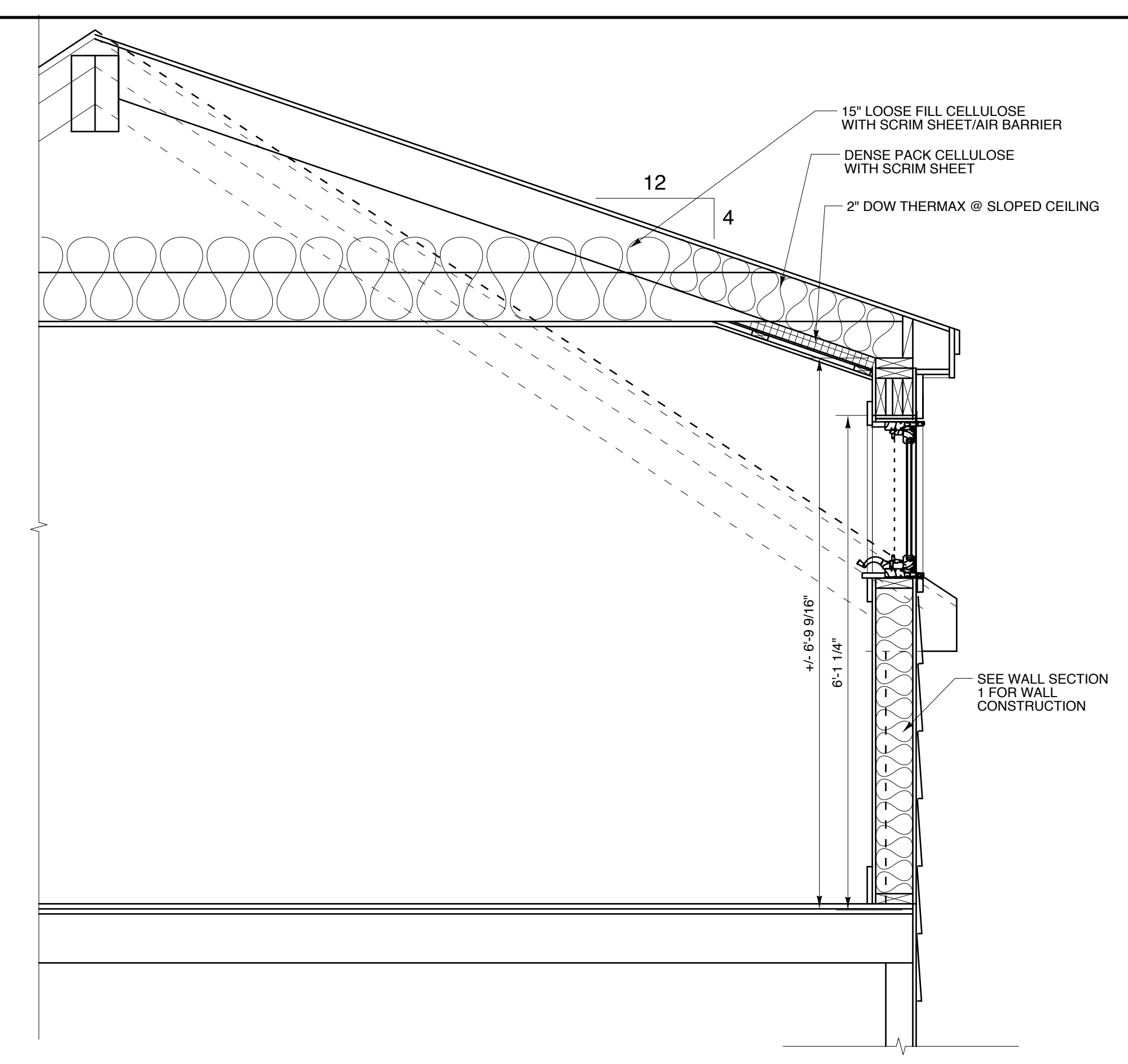
3 WALL SECTION @ GARAGE DORMER A300 SCALE: 3/4" = 1' - 0"
