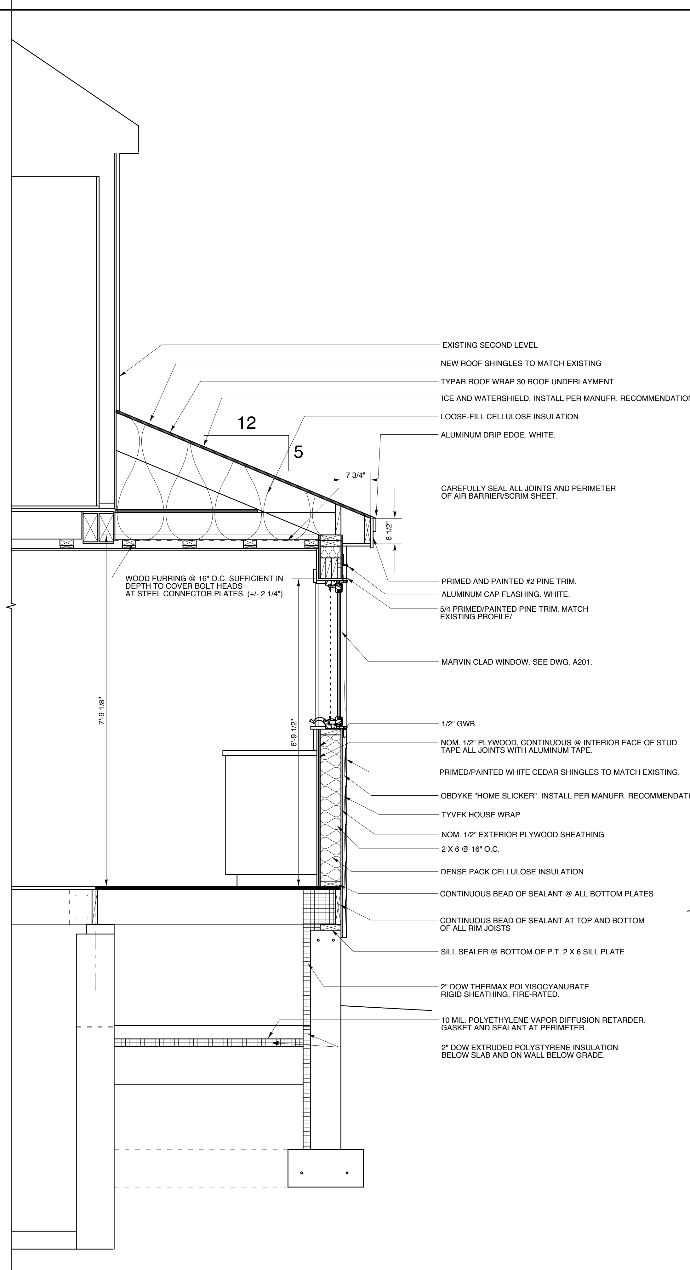
1 WALL SECTION @ KITCHEN A300 SCALE: 3/4" = 1' - 0"
