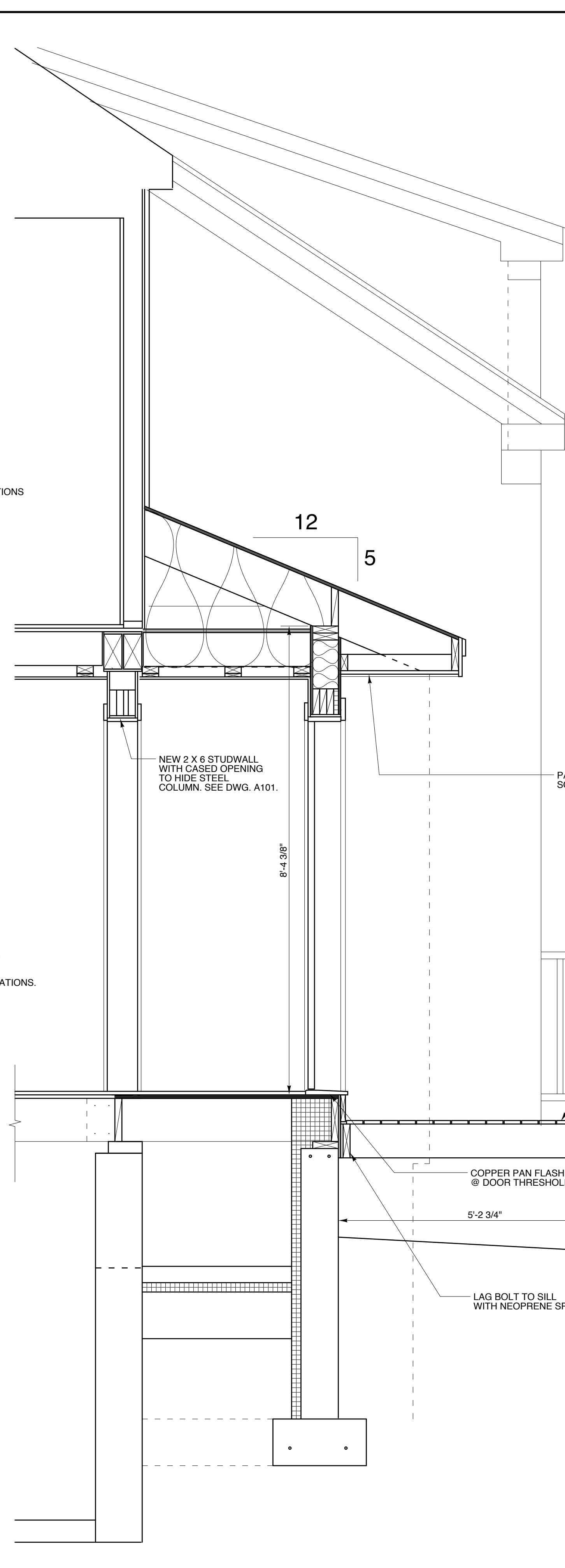
2 WALL SECTION @ DECK ENTRY A300 SCALE: 3/4" = 1' - 0"
