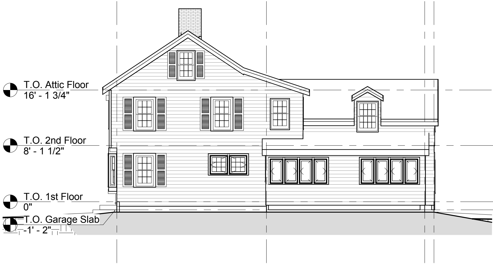
1 Existing Elevation - Side 1/8" = 1'-0"
