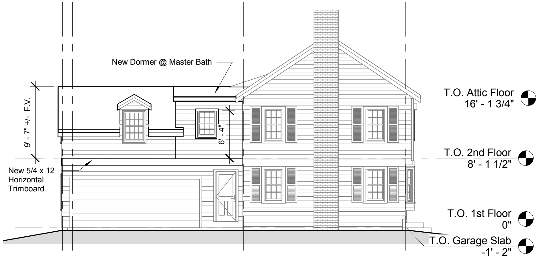
① LEFT ELEVATION 1/8" = 1'-0"
