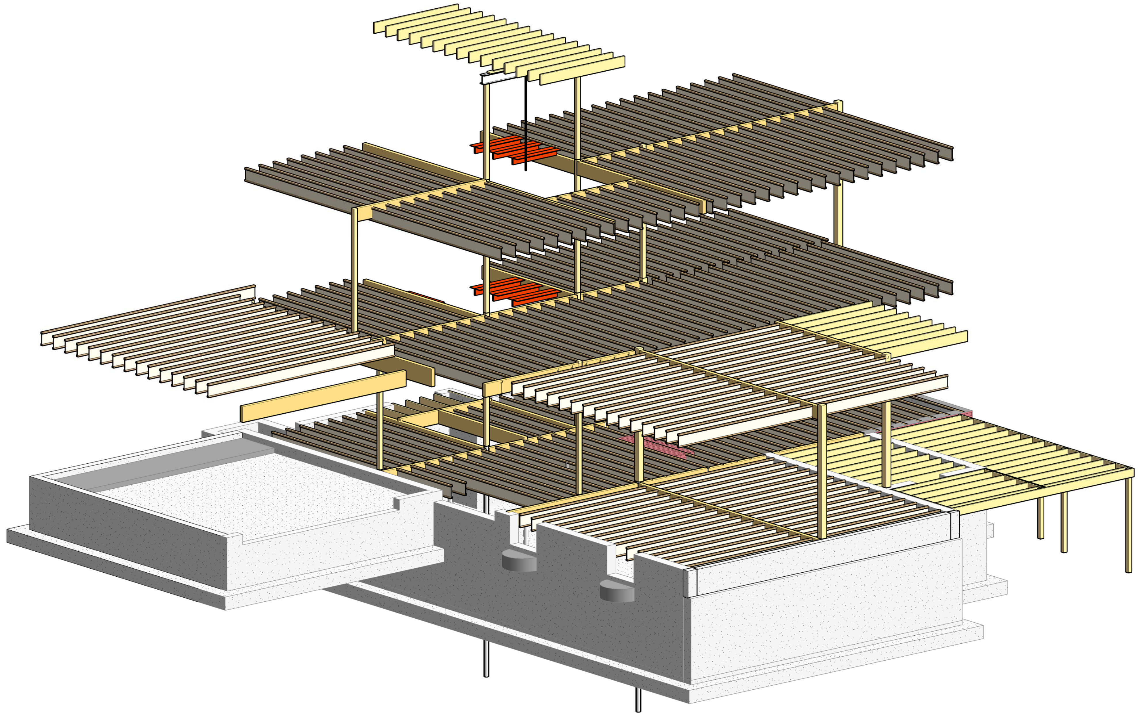
1 Structural Axonometric
