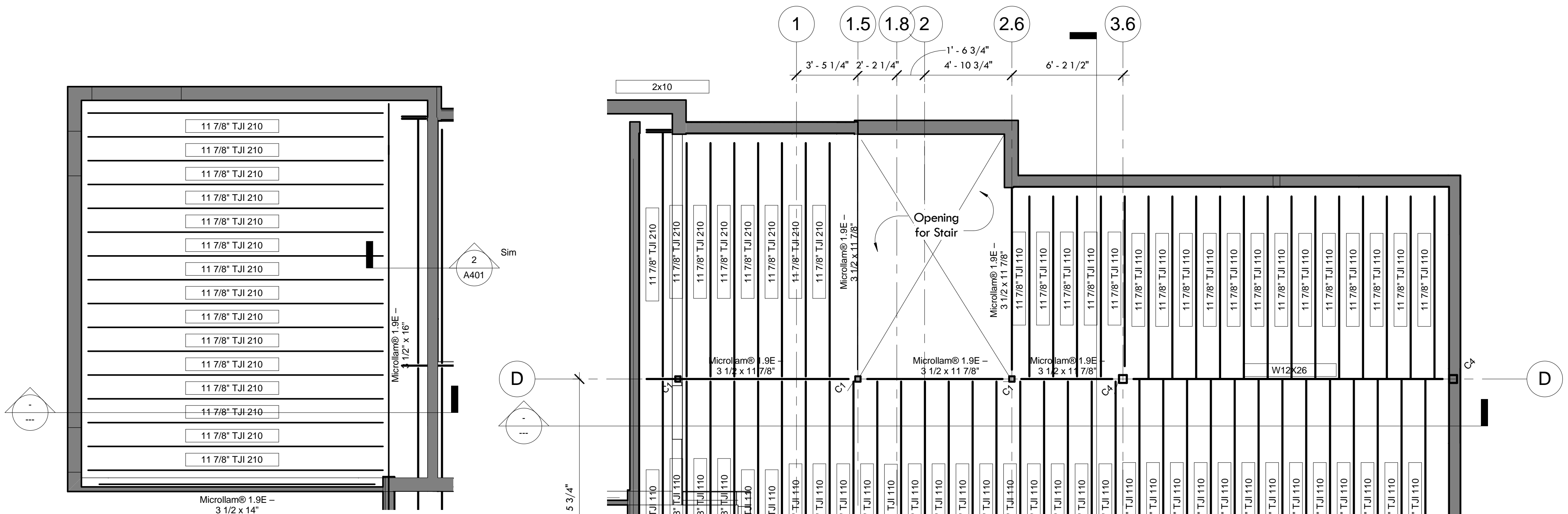
2 02.5 Garage Roof Framing 1/4" = 1'-0"
