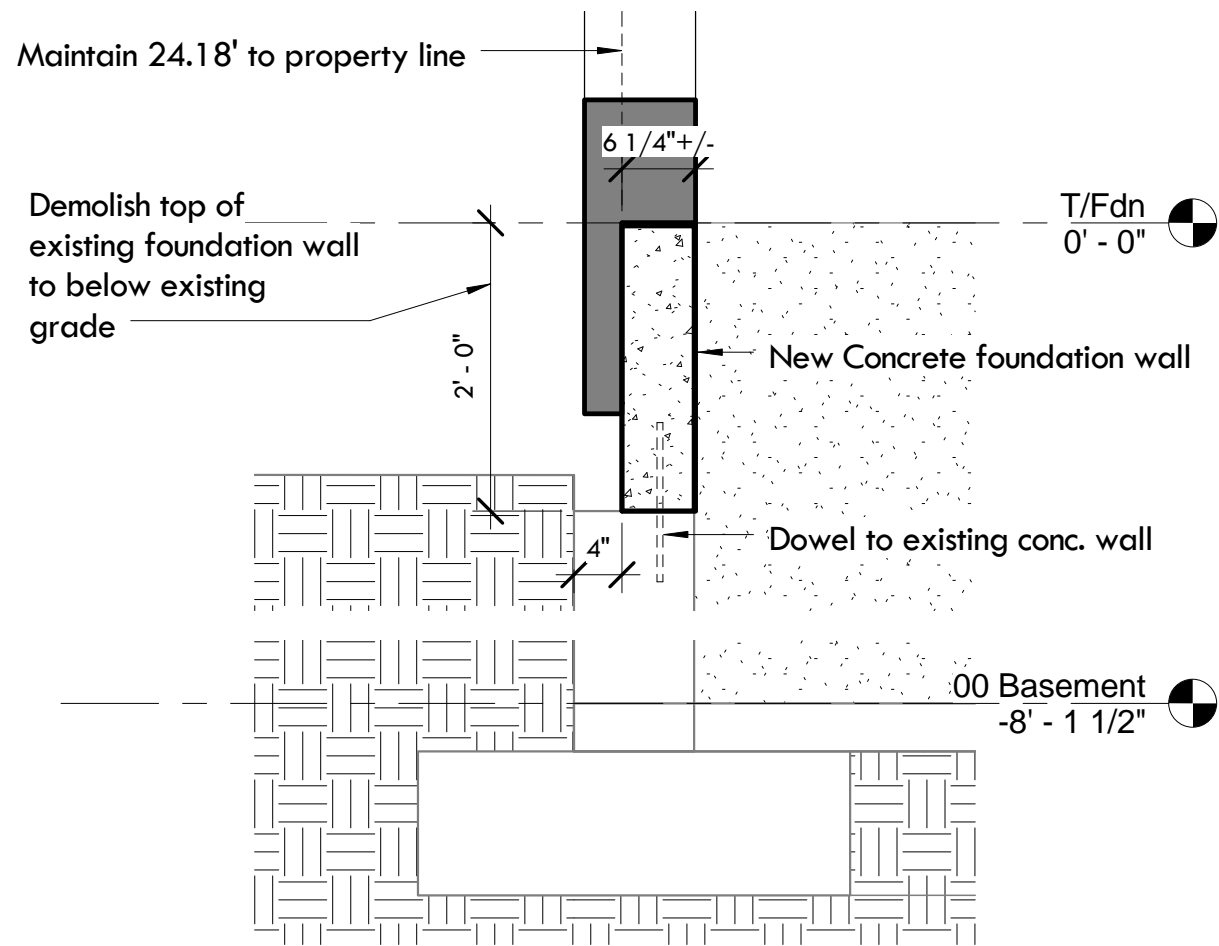
3 Foundation Wall Modifications 3/4" = 1'-0"
