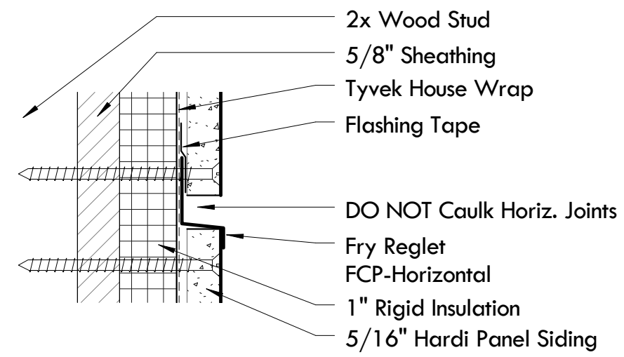
2 Reveal - Cement Panel - Horizontal 6" = 1'-0"
