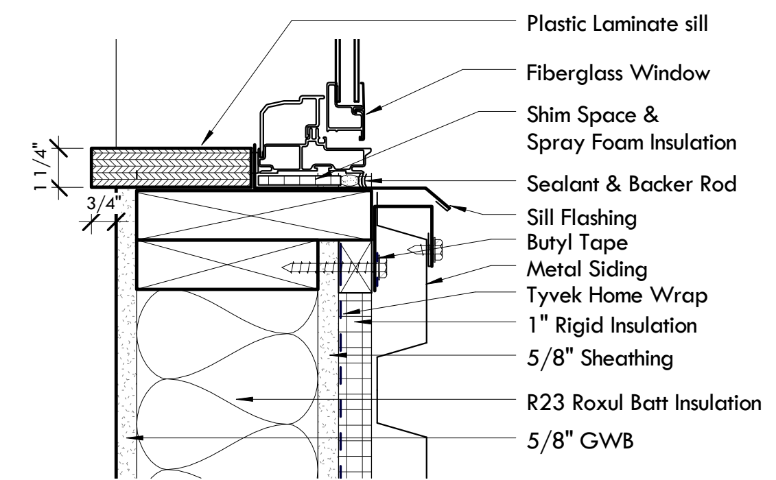
7 Sill @ Metal Siding Panel 3" = 1'-0"
