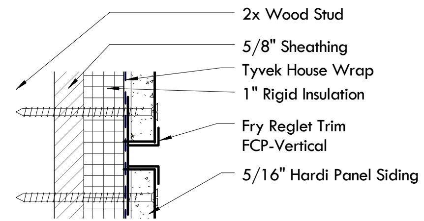
3 Reveal - Cement Panel - Vertical 6" = 1'-0"
