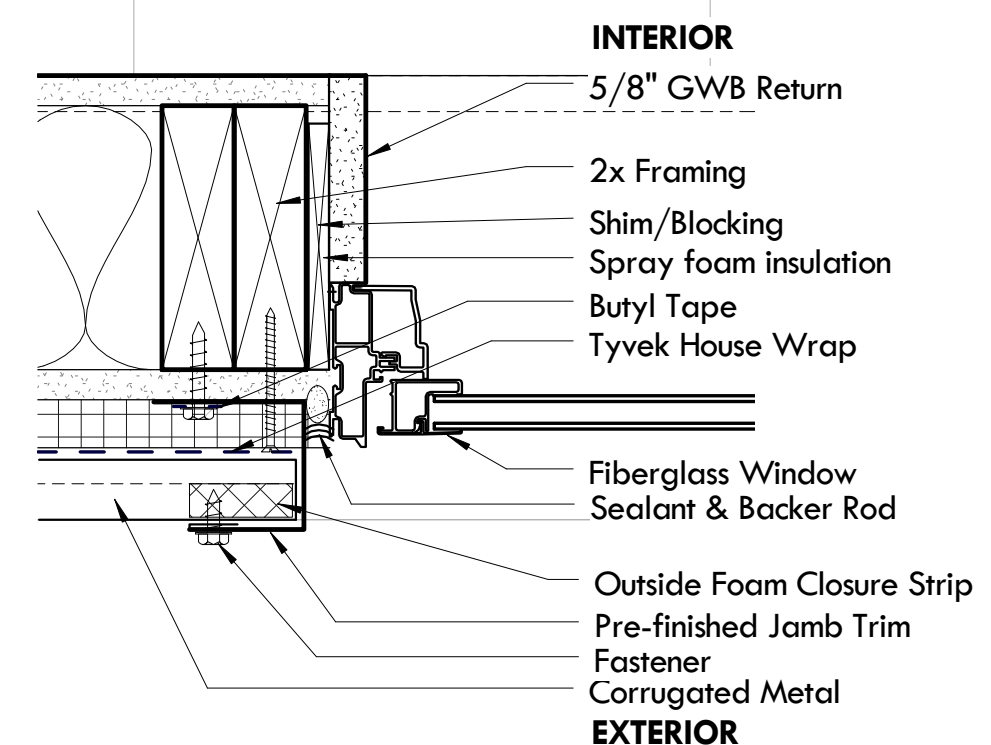
8 Jamb @ Metal Panel Siding 3" = 1'-0"
