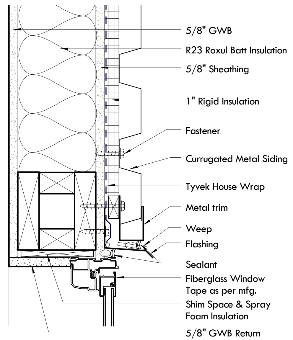
6 Head @ Metal Siding Panel 3" = 1'-0"
