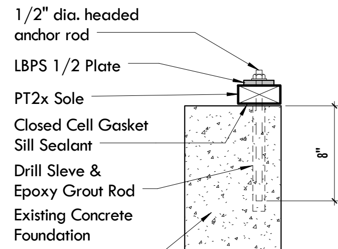
1 Callout of Section @ Garage 1 1/2" = 1'-0"
