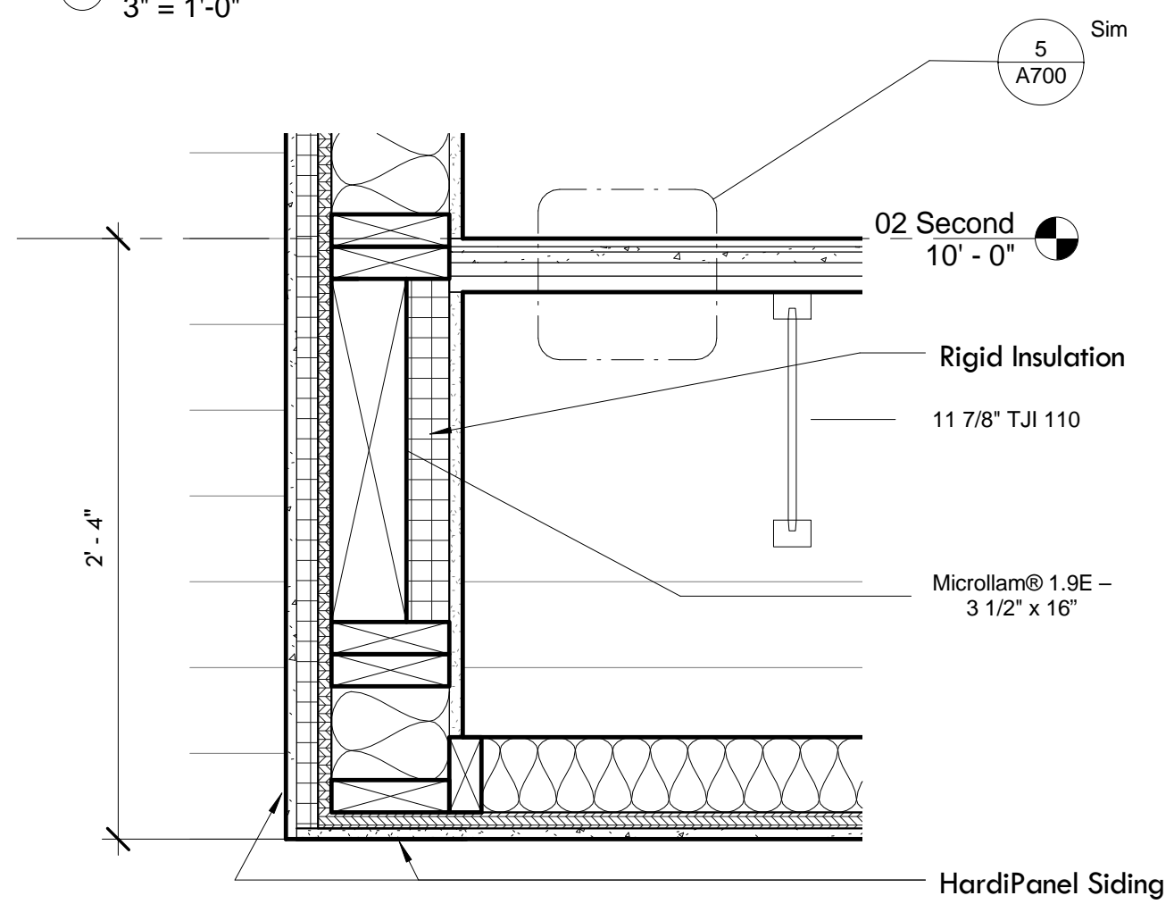
9 Callout of Wall Section @ Entrance 1 1/2" = 1'-0"
