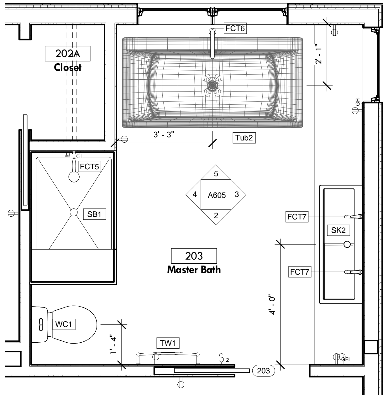
1 Bathroom - Master 1/2" = 1'-0"
