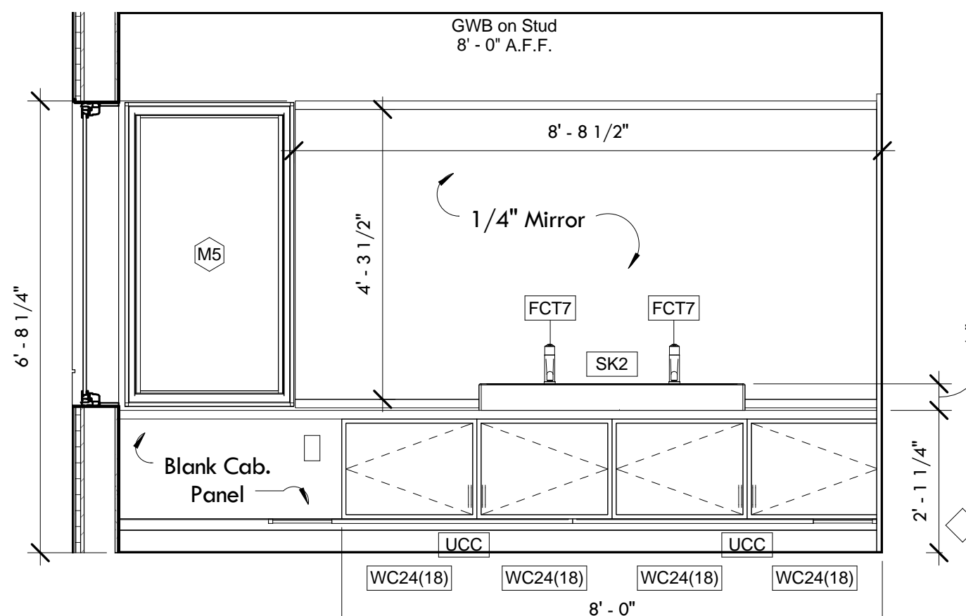
3 Master Bath - Sink 1/2" = 1'-0"
