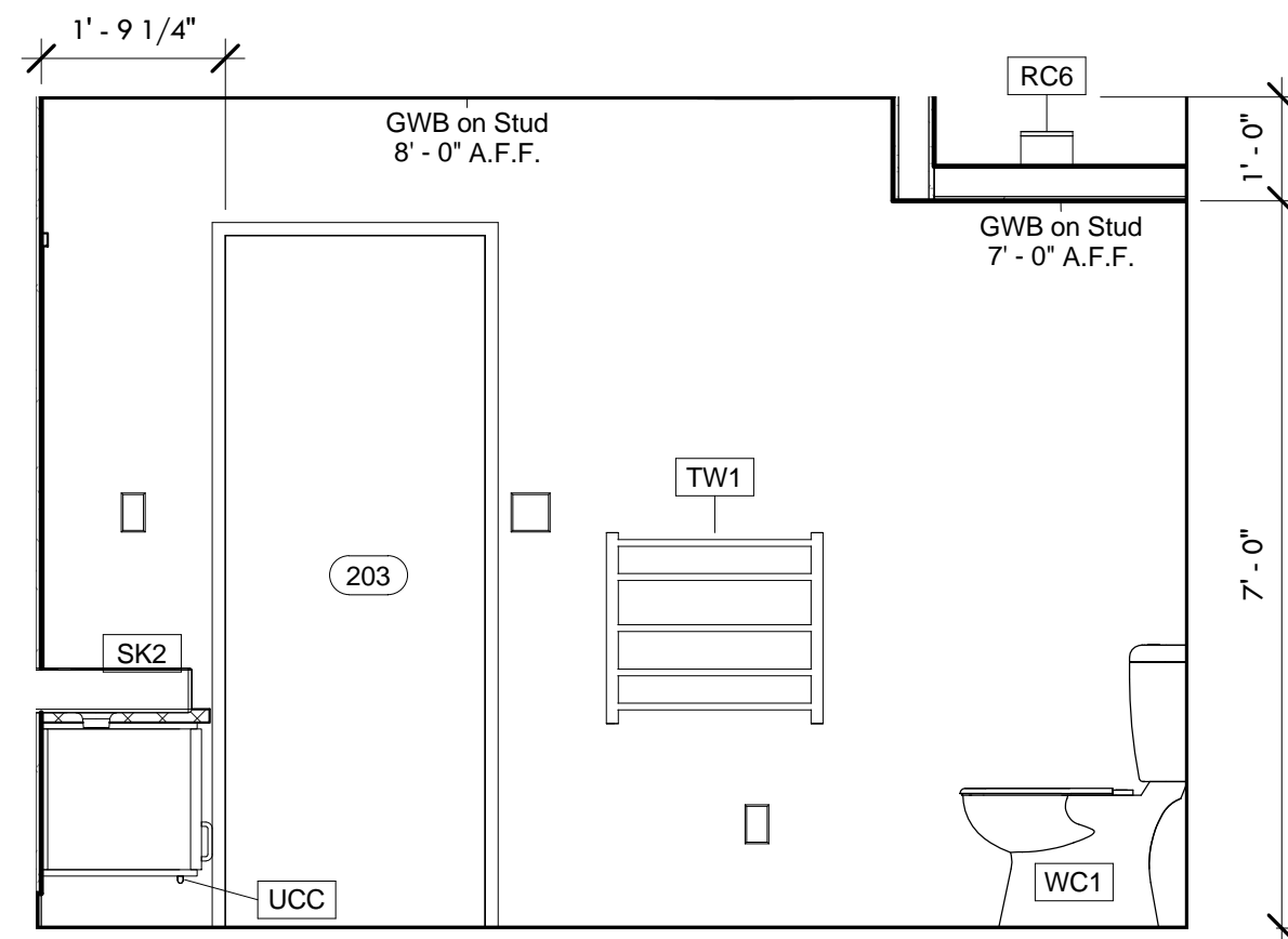
2 Master Bath - Door 1/2" = 1'-0"
