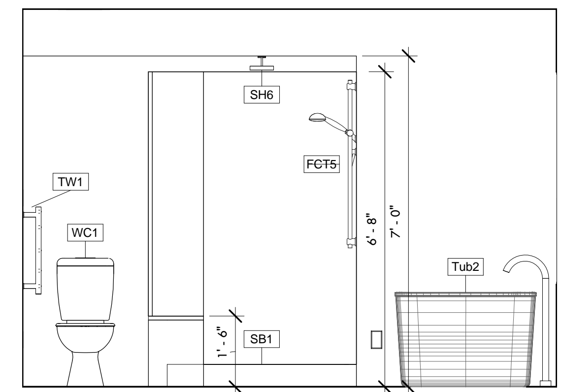
4 Master Bath - Toilet-Shower 1/2" = 1'-0"
