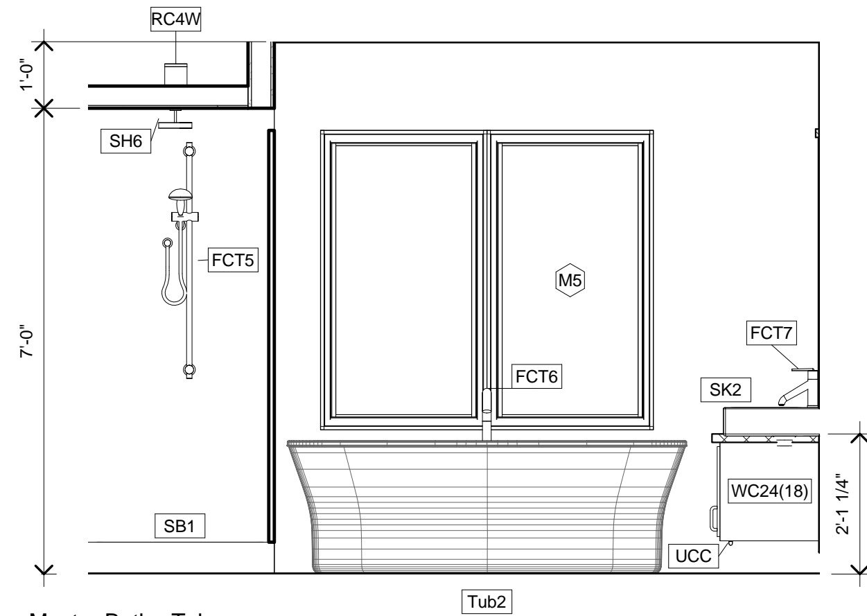
5 Master Bath - Tub 1/2" = 1'-0"
