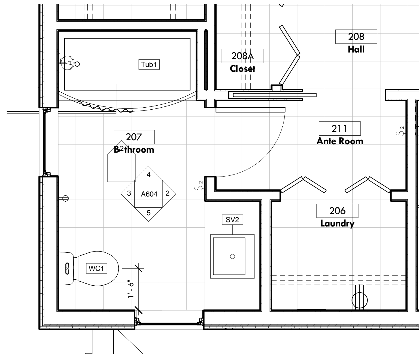
1 Bathroom - Second Floor 1/2" = 1'-0"
