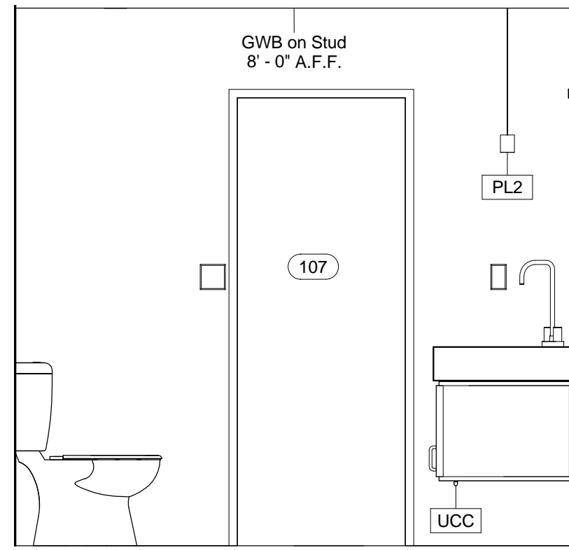
2 1st Flr Bath - Door 1/2" = 1'-0"
