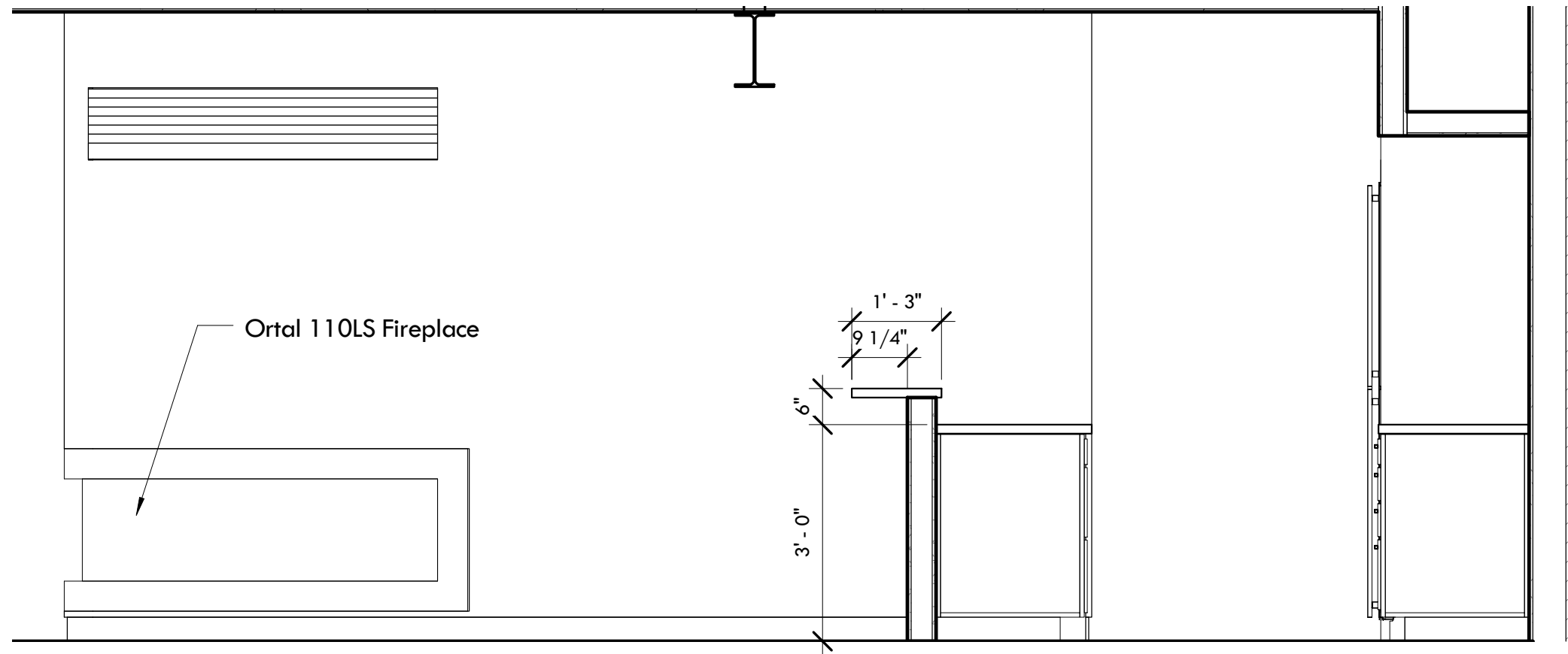
1 Kitchen - Section/Fireplace 1/2" = 1'-0"
