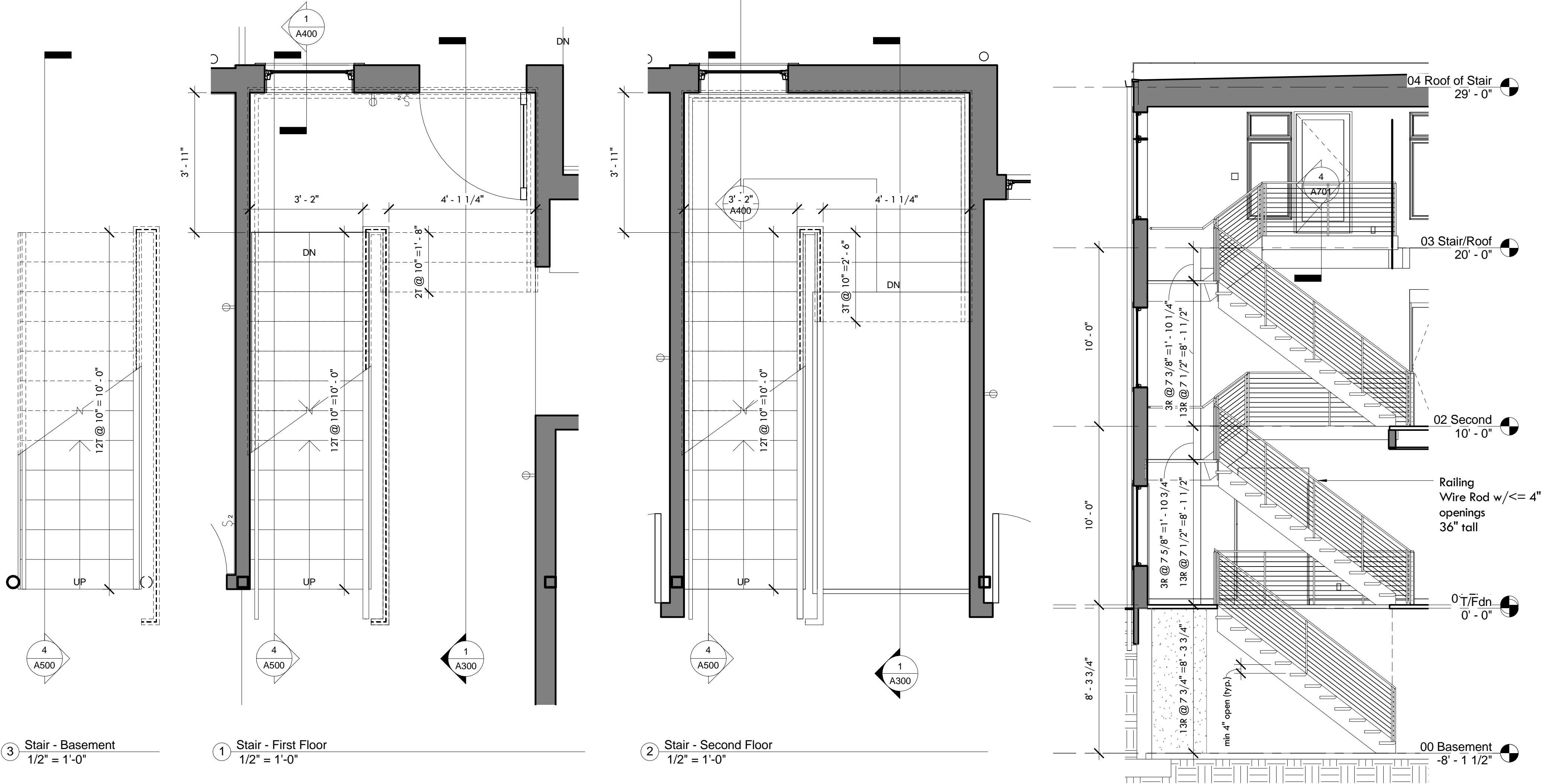
4 Section @ Stair 1/4" = 1'-0"
