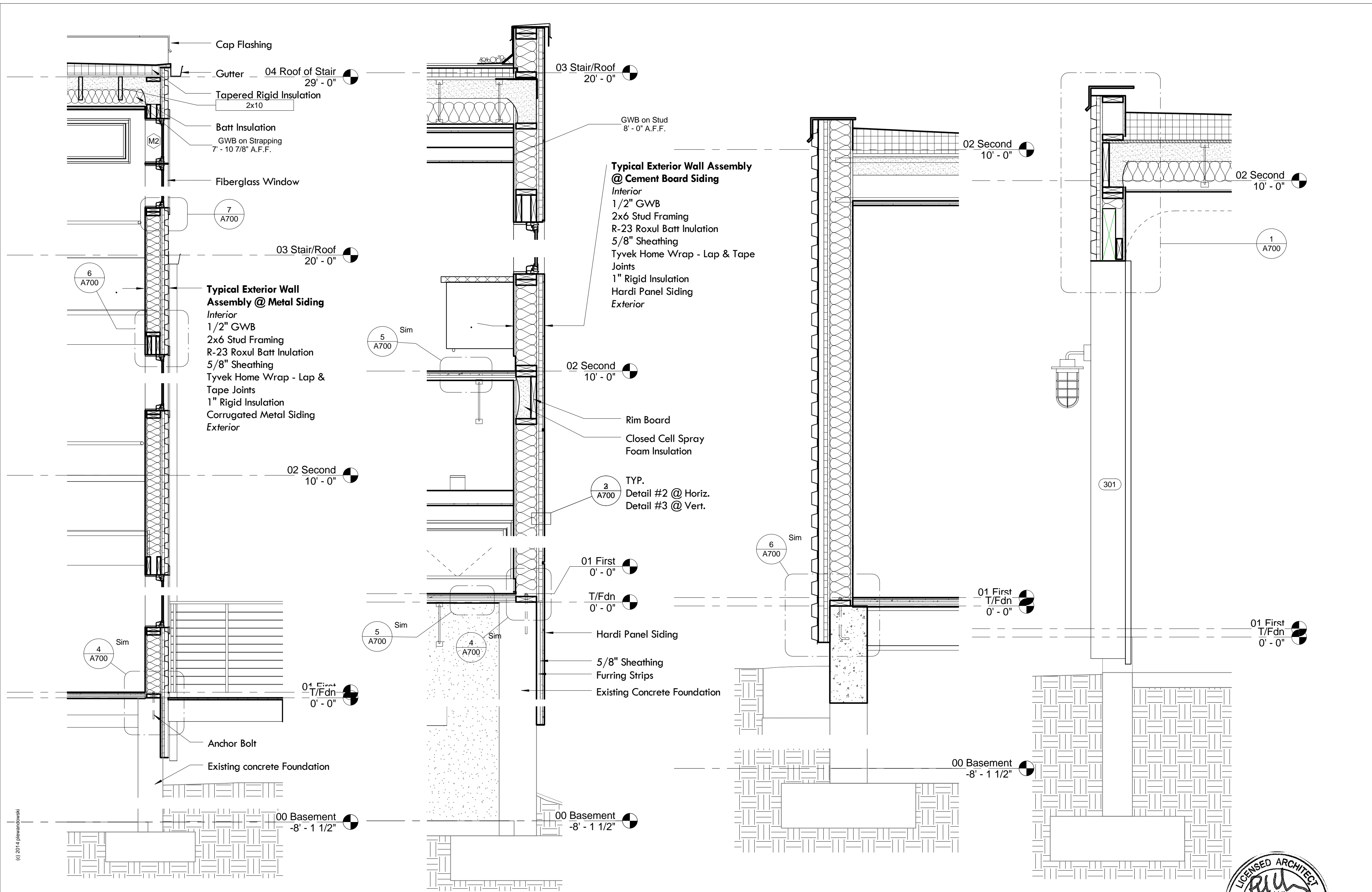
1 Wall Section @ Stair 1/2" = 1'-0"
