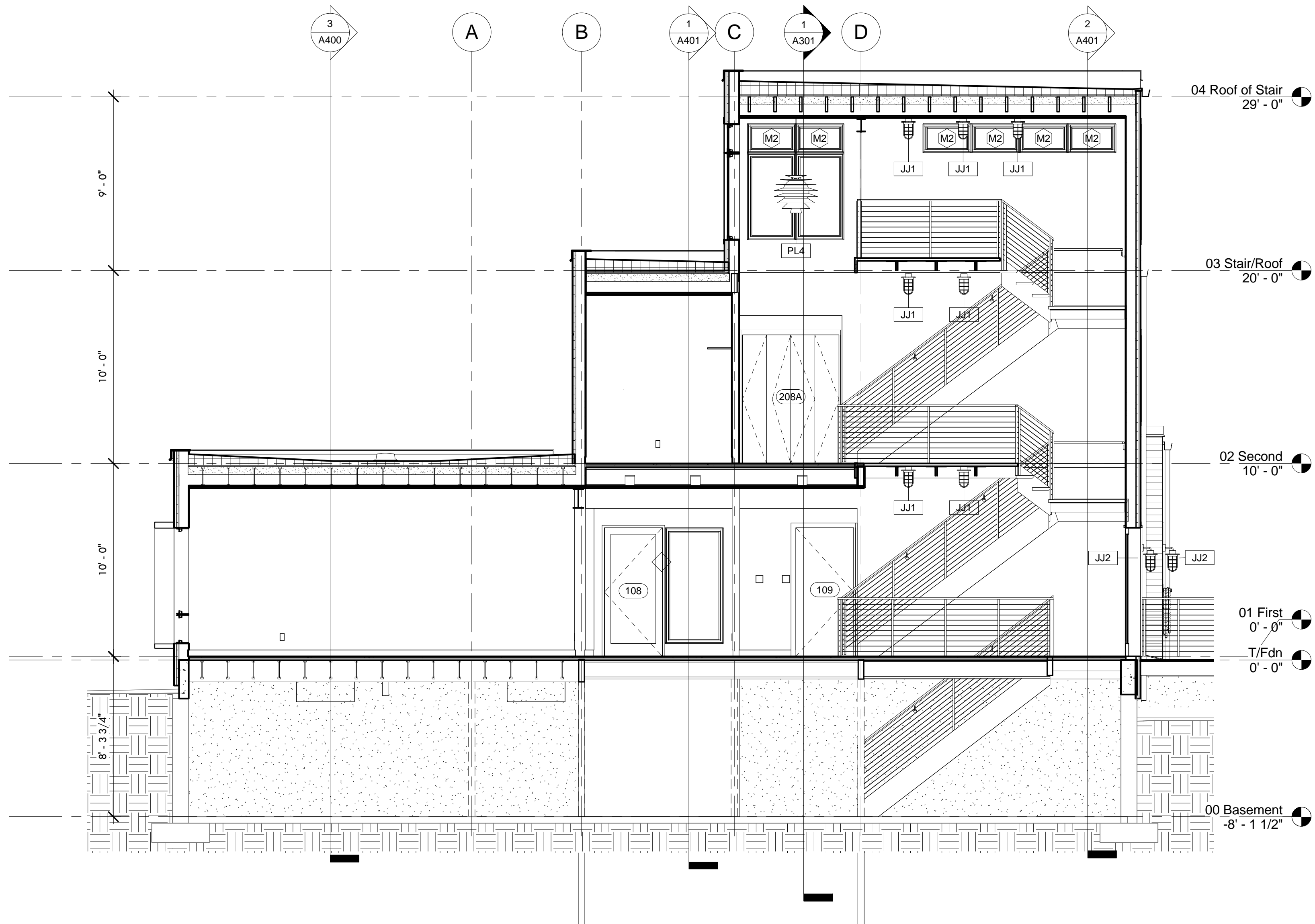
1 Transverse Section 1/4" = 1'-0"
