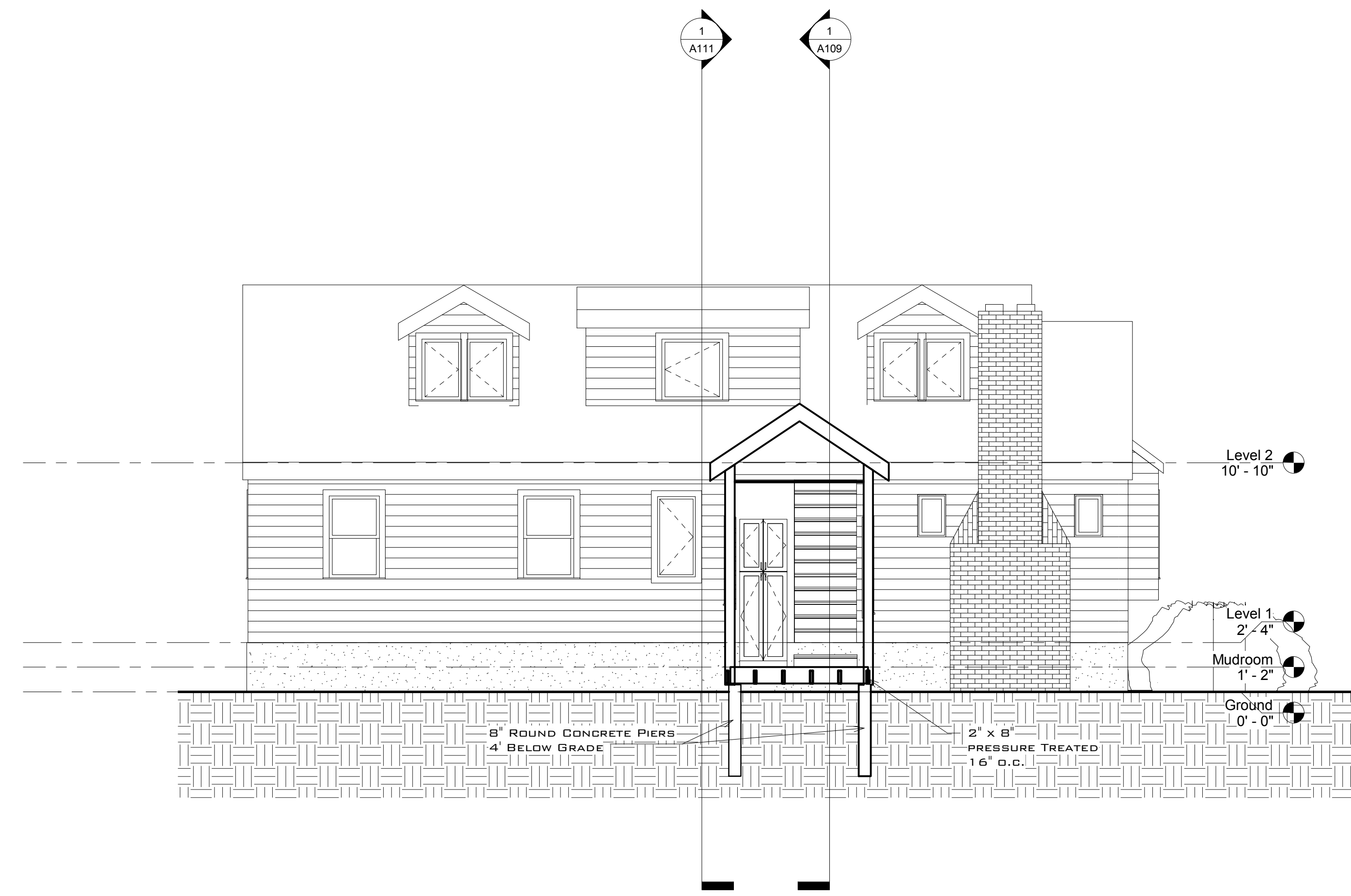
① Section 2 1/4" = 1'-0"
