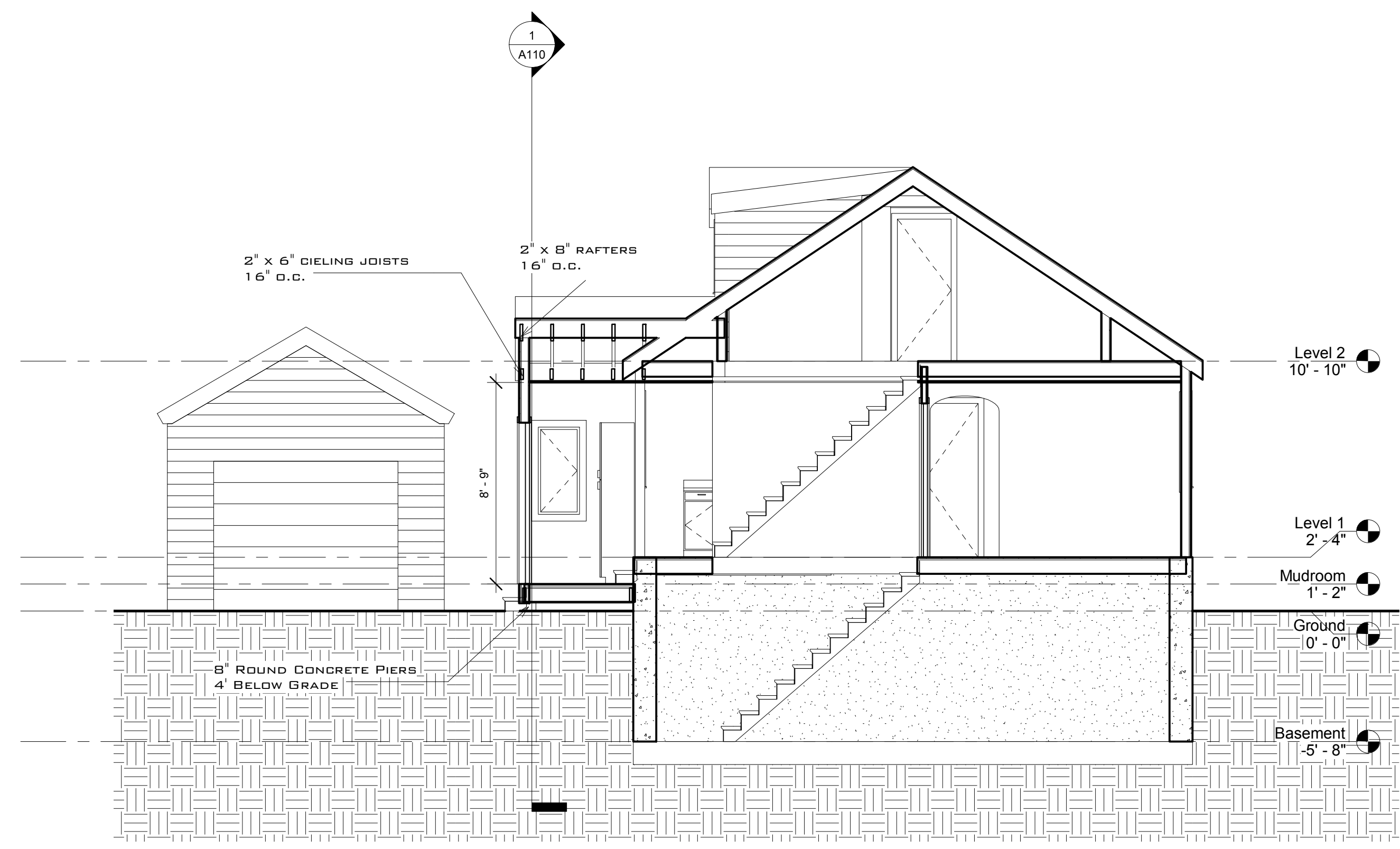
① Section 1 1/4" = 1'-0"
