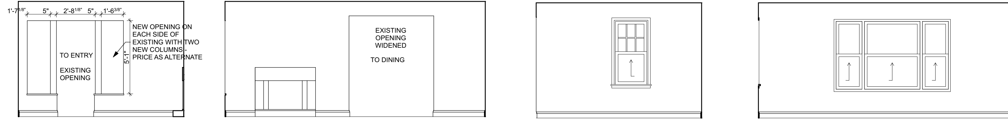
1 LIVING ROOM SCALE: 1/4" = 1'-0"
