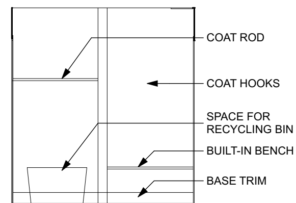
5 MUD ROOM SCALE: 1/4" = 1'-0"
