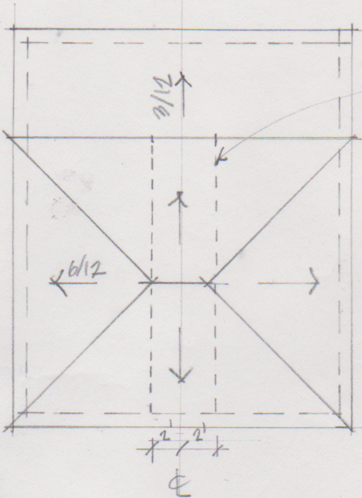
ROOF PLAN
