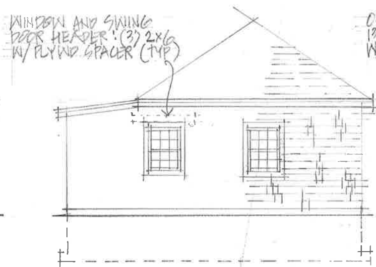
EAST ELEVATION
