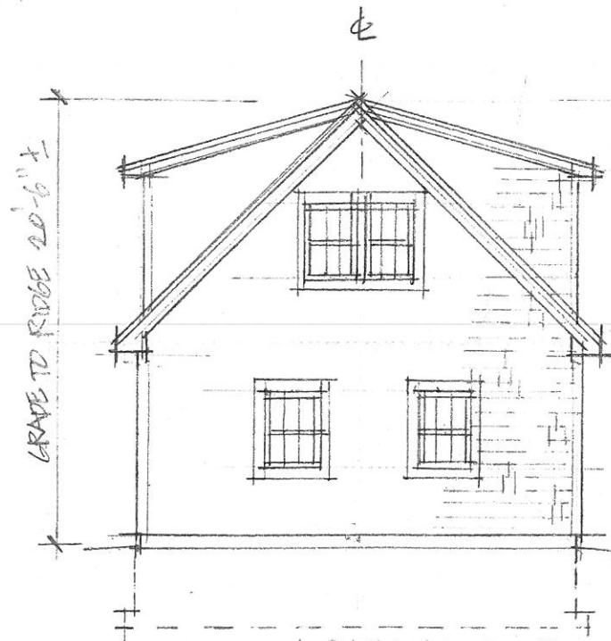
SOUTH ELEVATION
